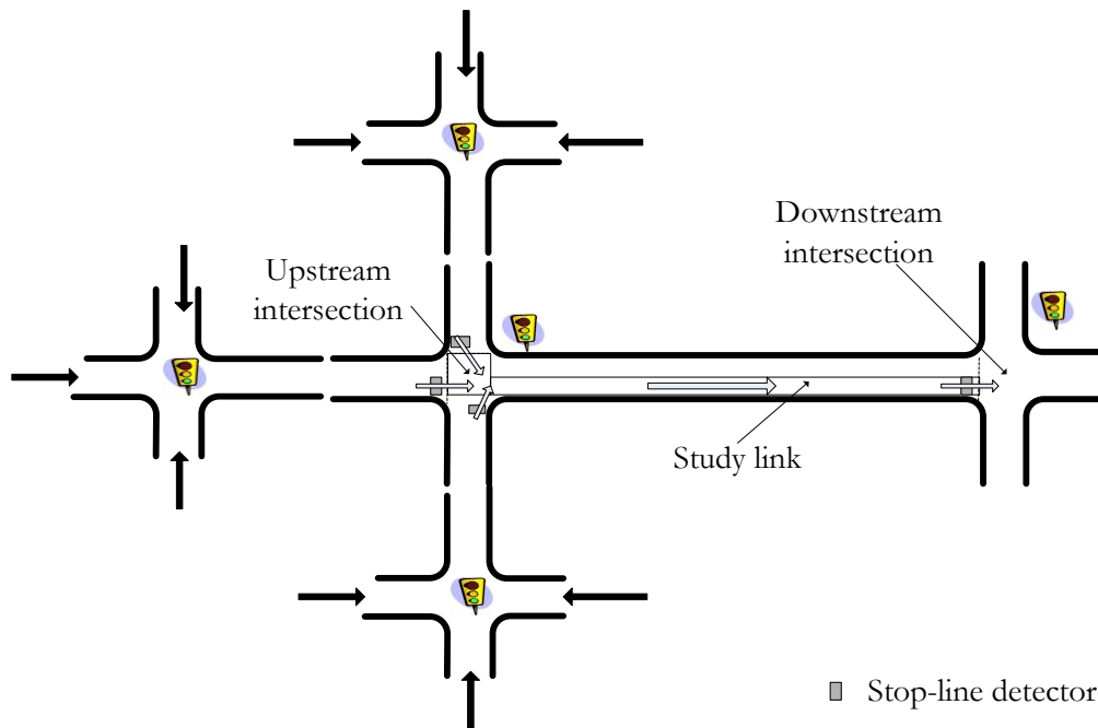
Figure 3-14: Test bed for model testing on a single link between two consecutive signalized intersections.
