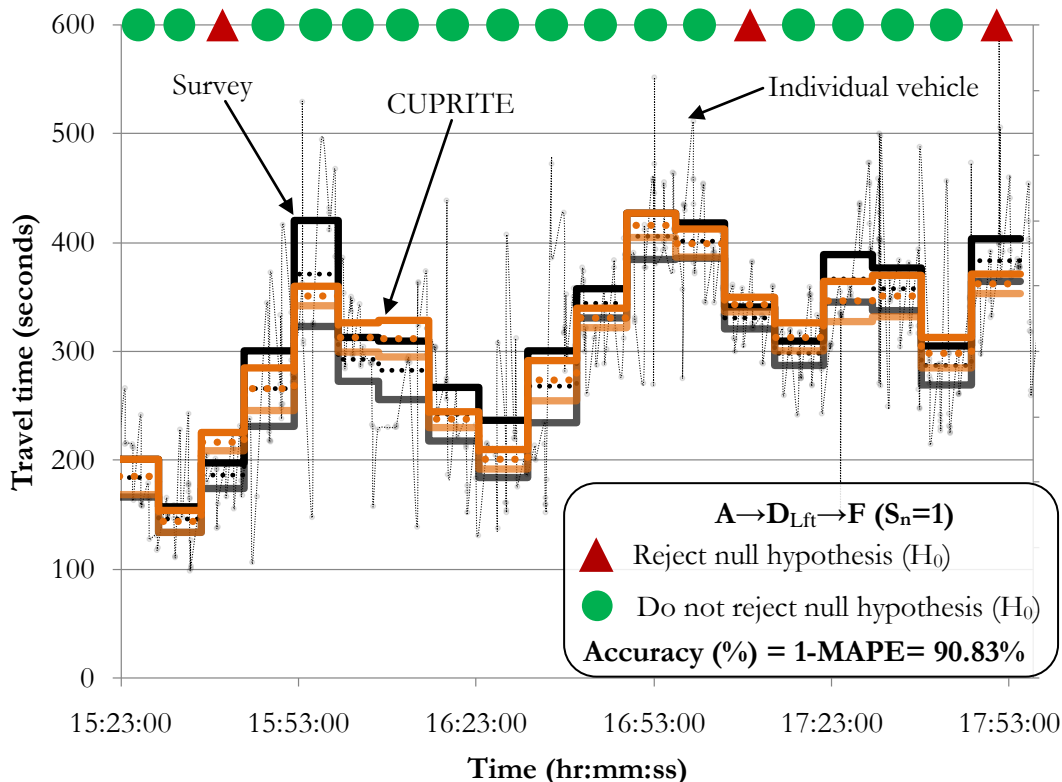
Figure D-4: Component based results for A→D Lft →F (S n =1).
