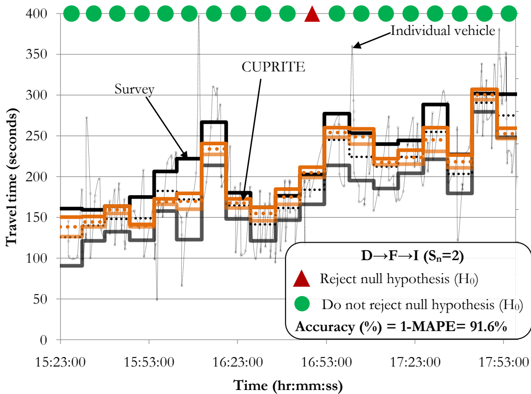
Figure E-6: Component based results for D→F→I ( S_n=2 ).
