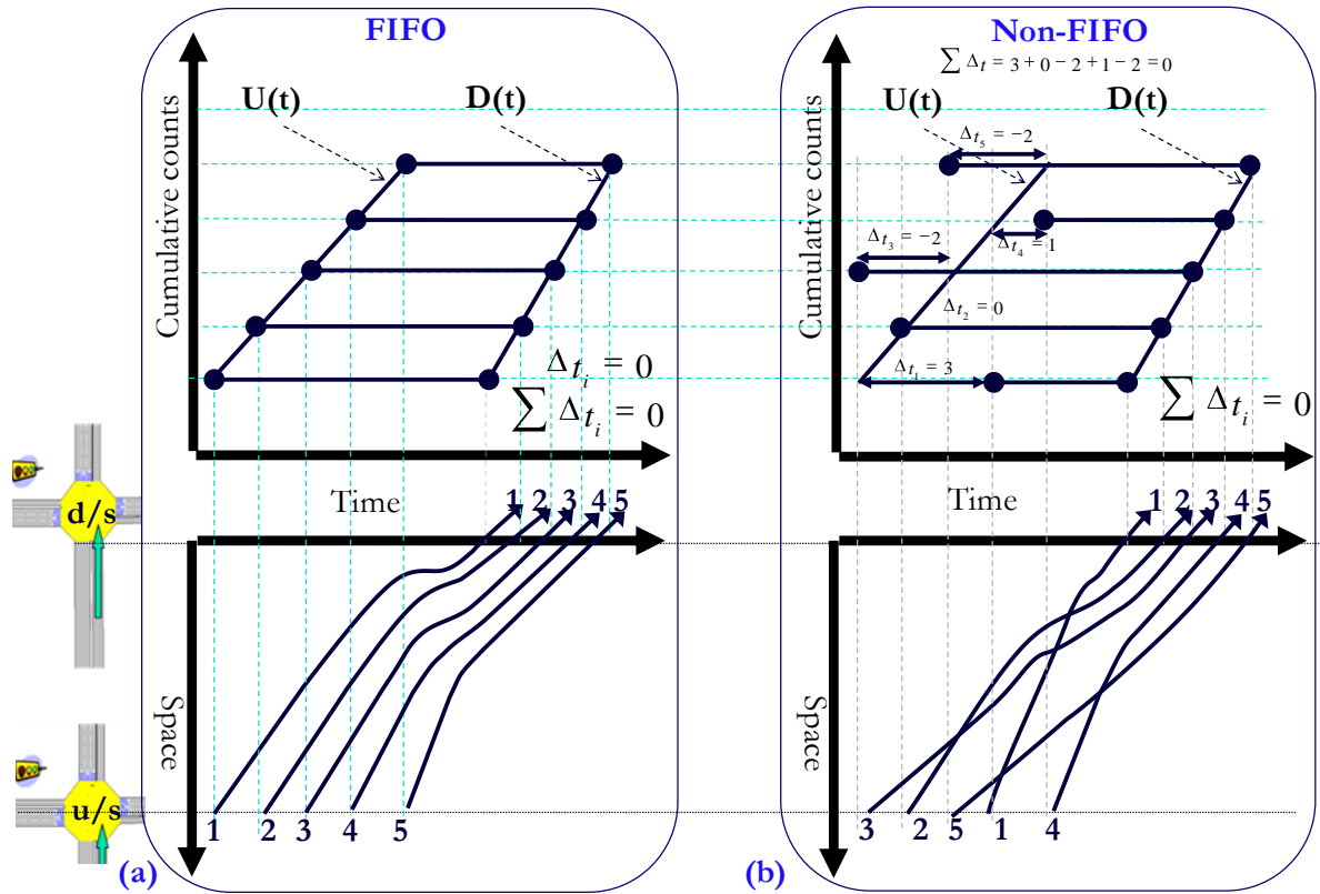
Figure 3-3: Relation between probe data (vehicle space-time trajectory) and cumulative plots for FIFO and non-FIFO situation.
