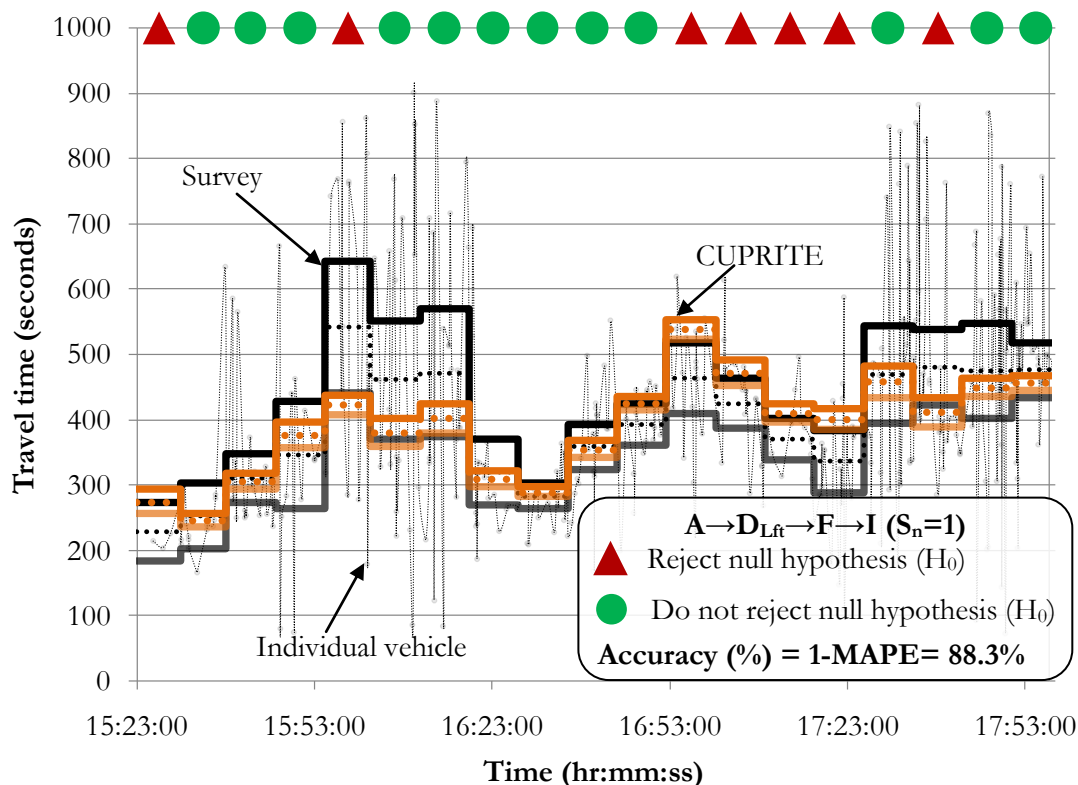
Figure G-4: Component based results for A→D Lft →F→I ( S_n=1 ).
