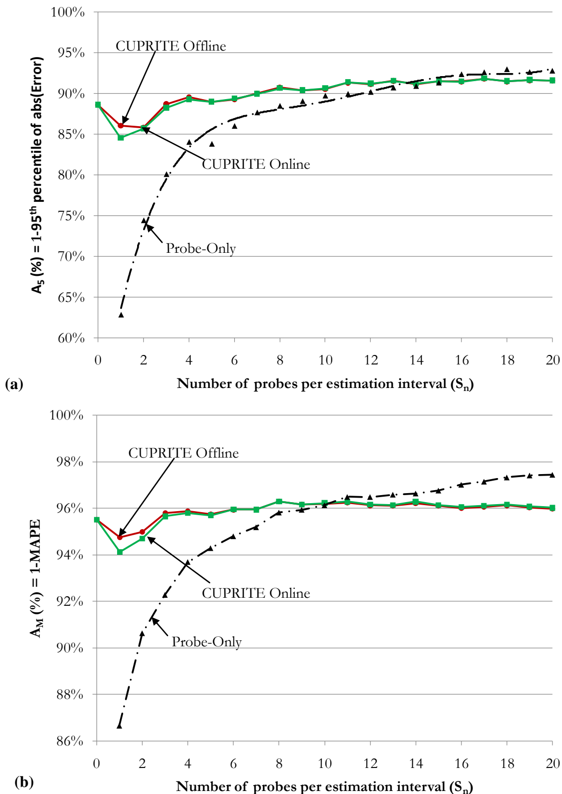
Figure C-13: Simultaneous presence of both sink and source. Case B4.3 (10% sink and 10% source): (a) A_5 and (b) A_M versus S_n .
