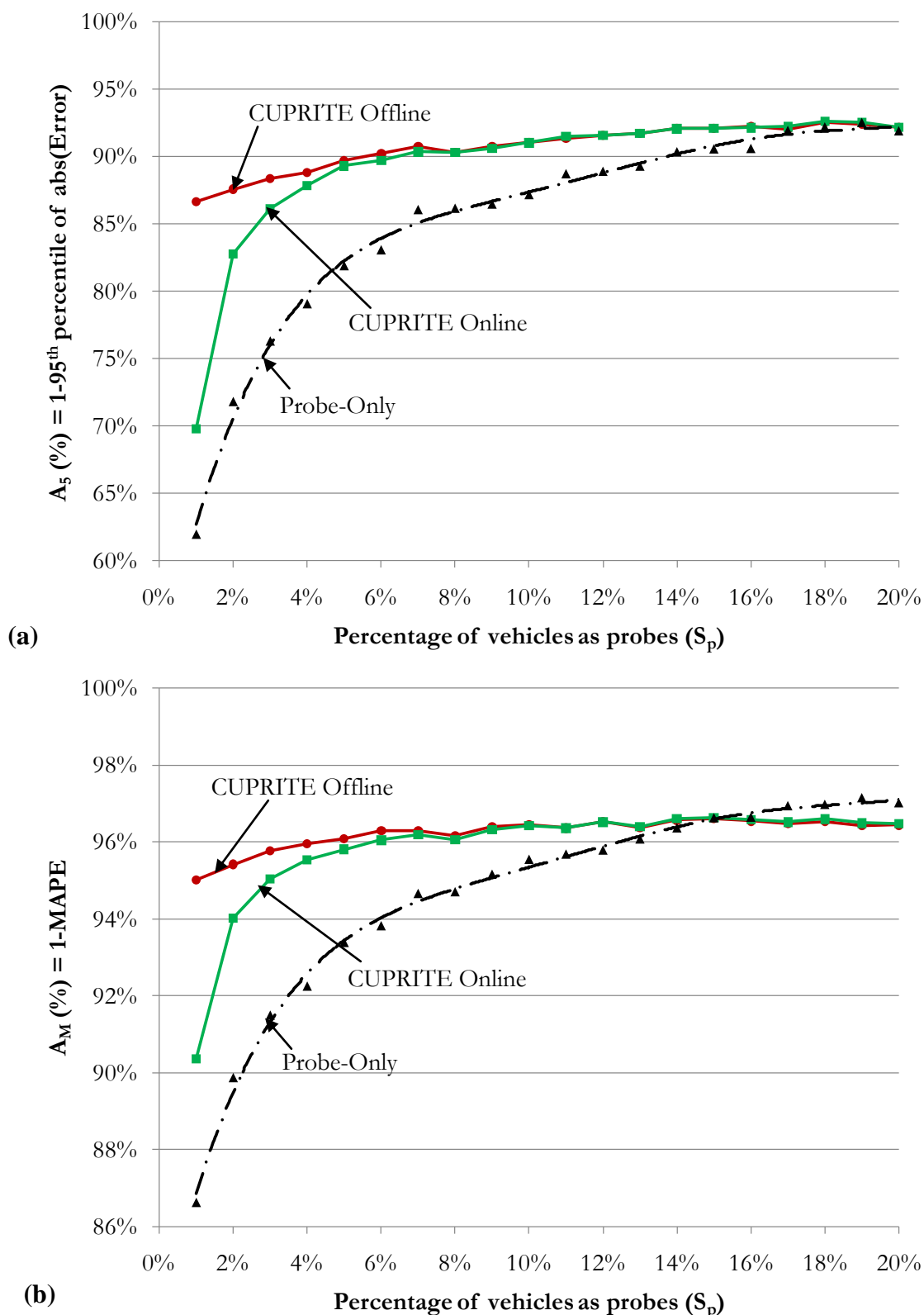
Figure 3-30: 10% sink case results for accuracy: a) A_5 and b) A_M versus S_p .
