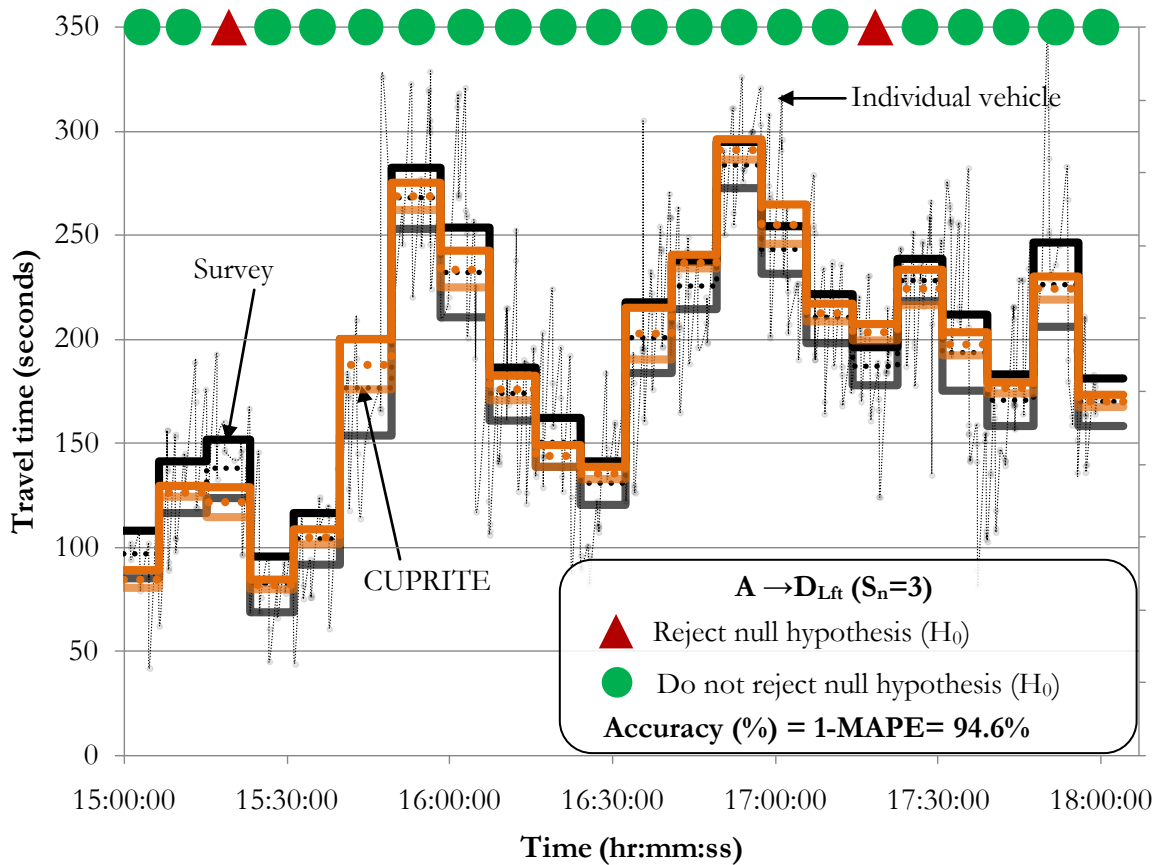
Figure 5-18: Results for A \rightarrow D_{Lft} with S_n = 3 .
