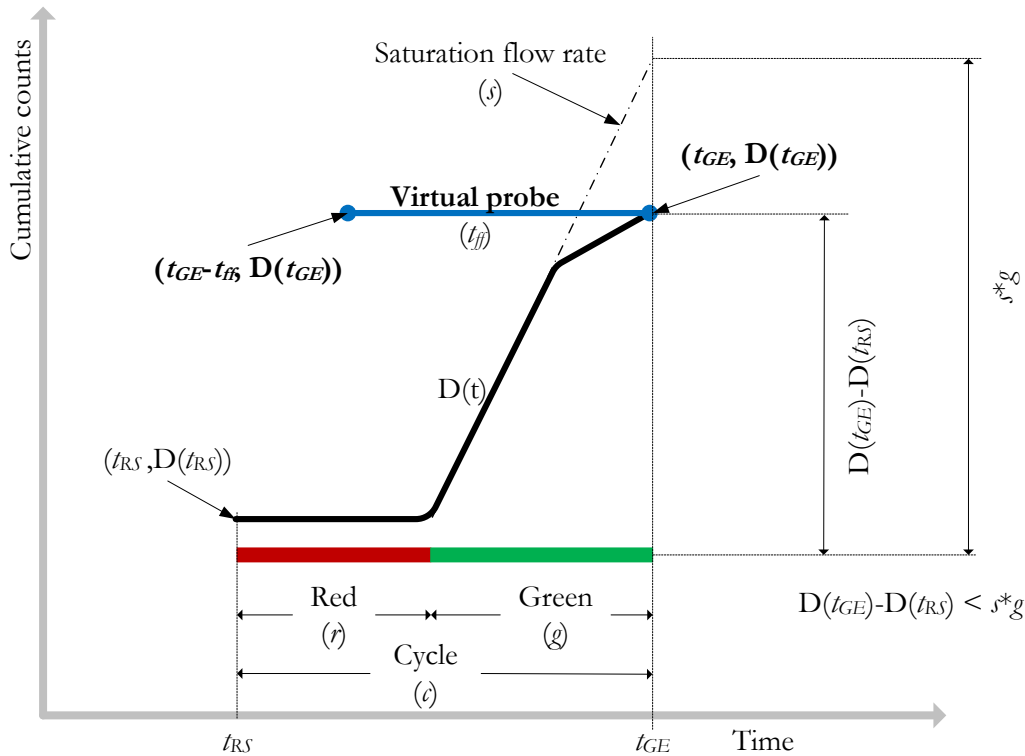
Figure 3-4: Illustration of virtual probe, fixed to D(t) at the end of signal green phase.
