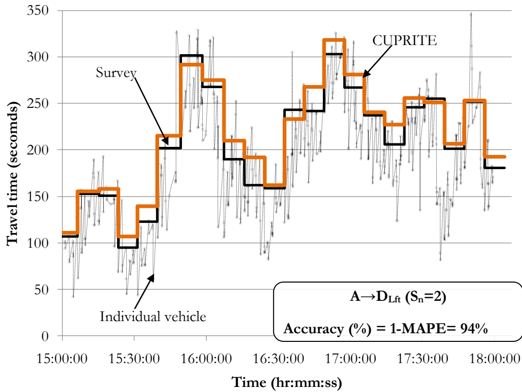
Figure H-4: Q_3 estimation using CUPRITE for route from A \rightarrow D Lft ( S_n=2 ).
