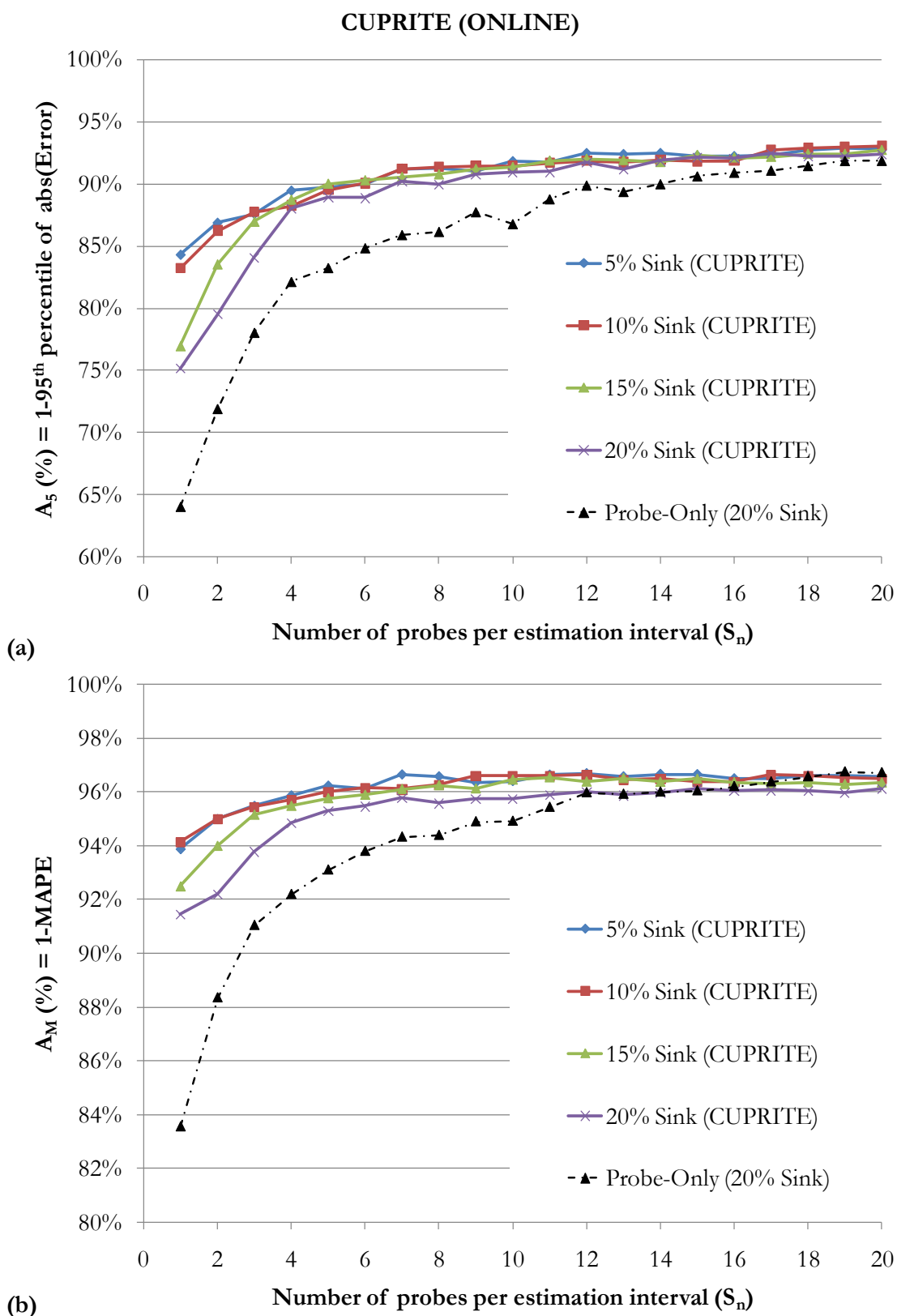
Figure 3-24: CUPRITE Online application for different sink percentages (5%, 10%, 15% and 20%); oversaturated traffic condition; non-FIFO discipline Results for accuracy: a) A_5 and b) A_M versus S_n .
