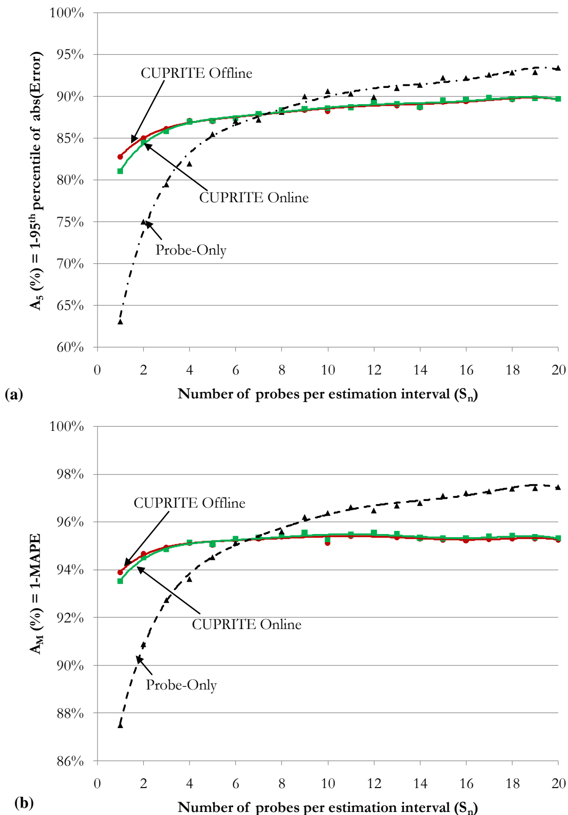
Figure C-10: Simultaneous presence of both sink and source. Case B4.2 (10% sink and 20% source): (a) A_5 and (b) A_M versus S_n .
