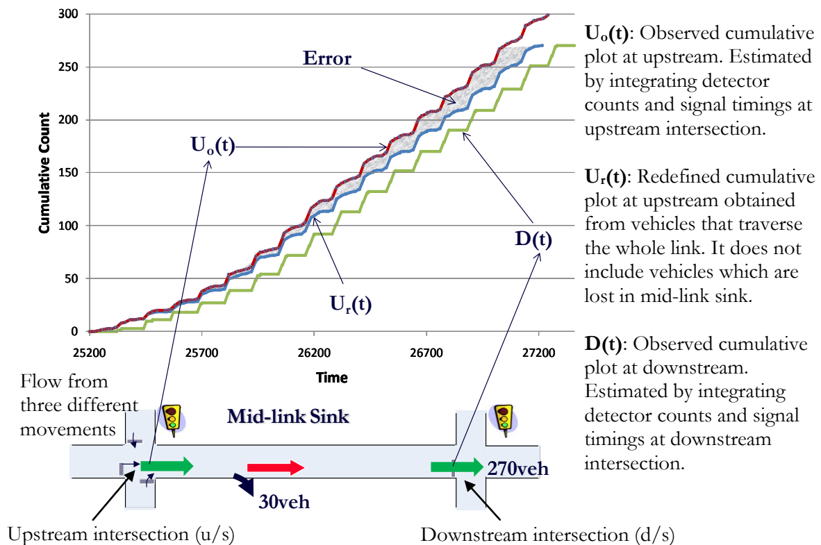
Figure 3-1: Illustration of the effect of mid-link sink on classical analytical procedure.
