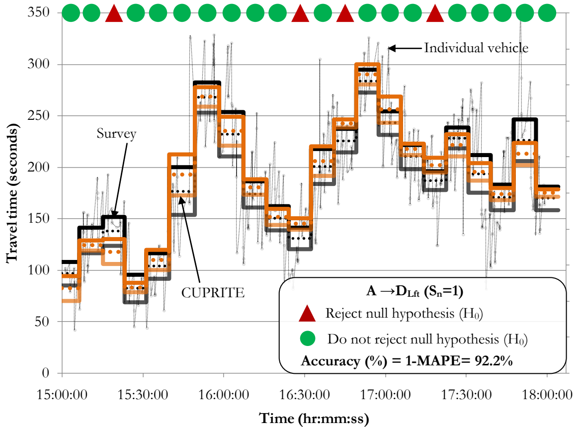
Figure 5-16: Results for A \rightarrow D_{Lft} with S_n = 1 .
