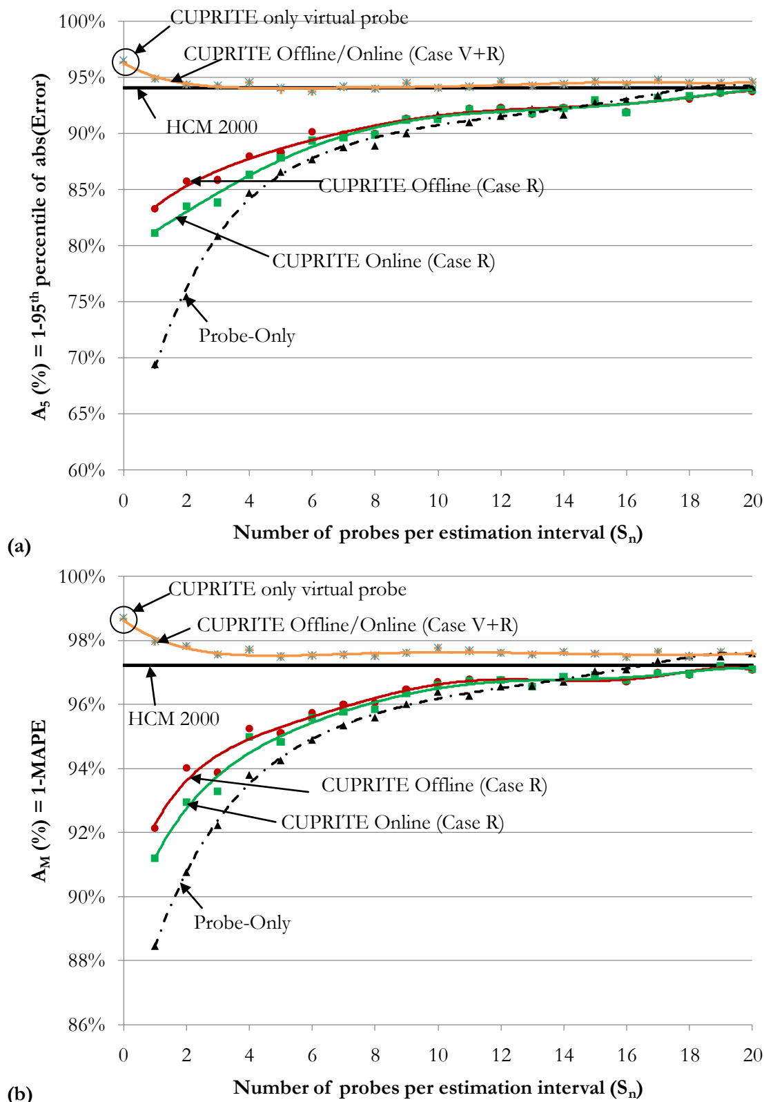
Figure C-4: Comparative results for 10% downstream detector undercounting case during undersaturated traffic condition. Results for accuracy: (a) A_5 and (b) A_M versus S_n .
