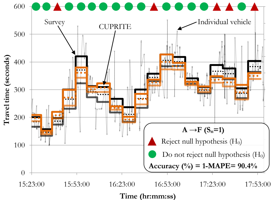
Figure D-1: Extreme based results for A→F (S n =1).
