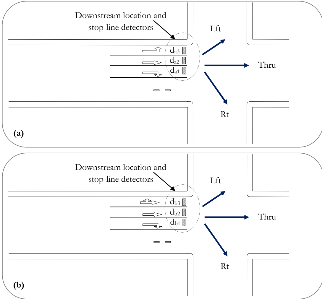
Figure 4-3: Example for two different downstream exit movement combinations based on link geometry.
