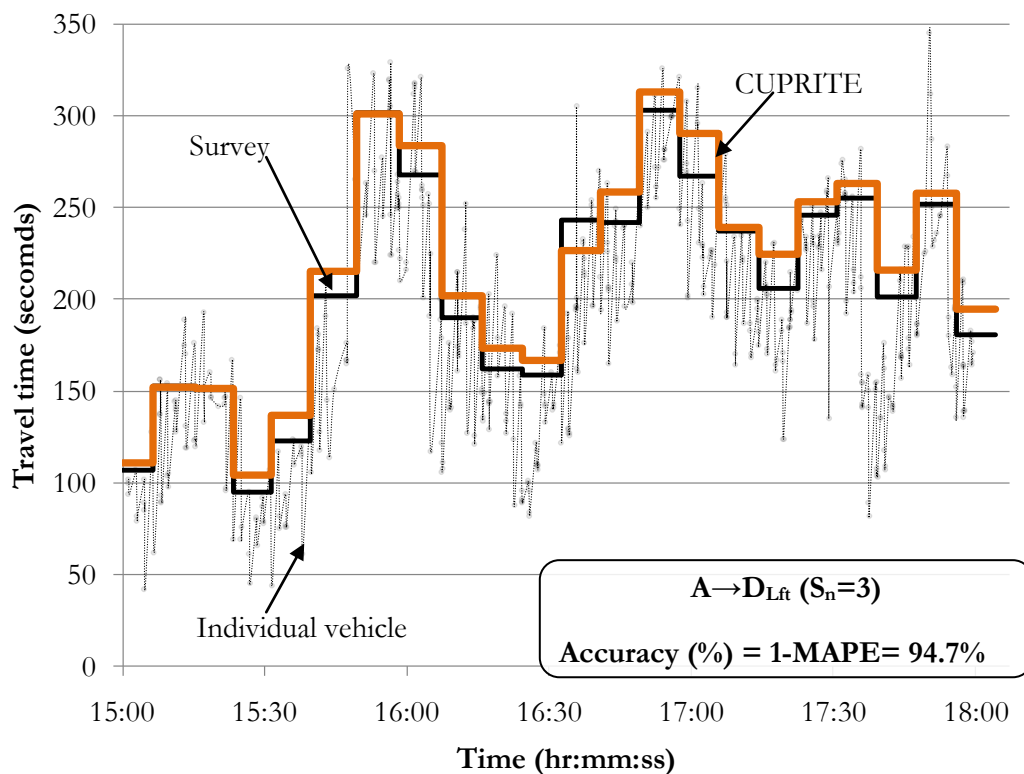
Figure H-5: Q_3 estimation using CUPRITE for route from A \rightarrow D Lft ( S_n=3 ).
