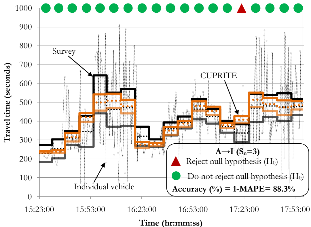
Figure G-3: Extreme based results for A→I ( S_n=3 ).
