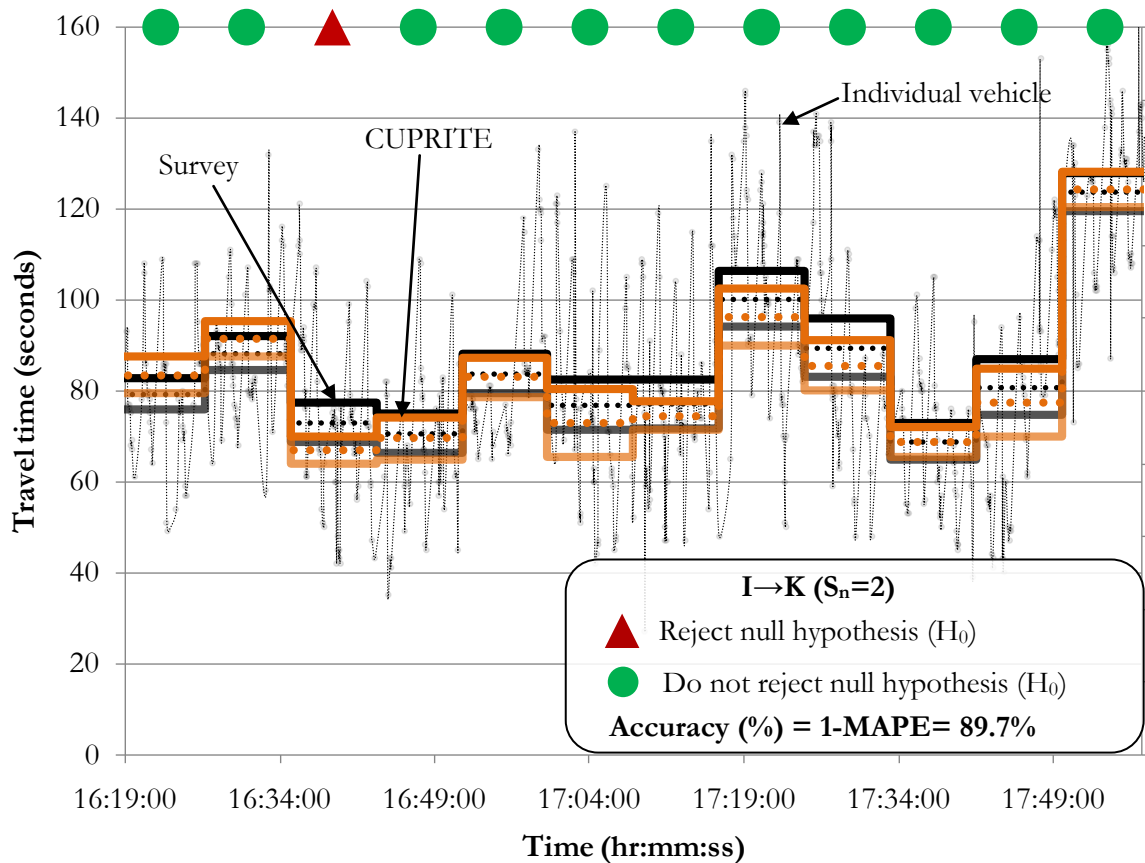
Figure 5-26: Results for I→K with S_n = 2 .
