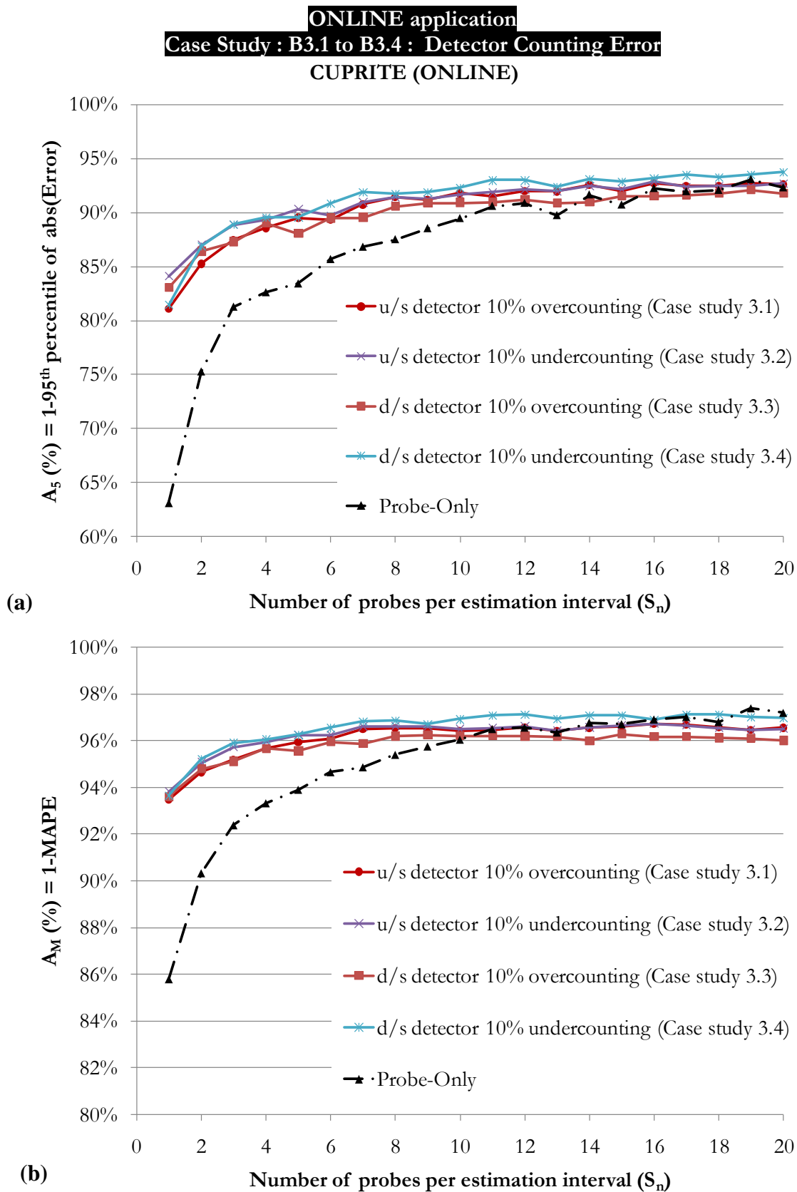
Figure C-8: Detector counting error with fixed number of probes per estimation interval ( S_n ) for Online application: Case B3. 1 to B3.4: (a) A_5 and (b) A_M versus S_n .
