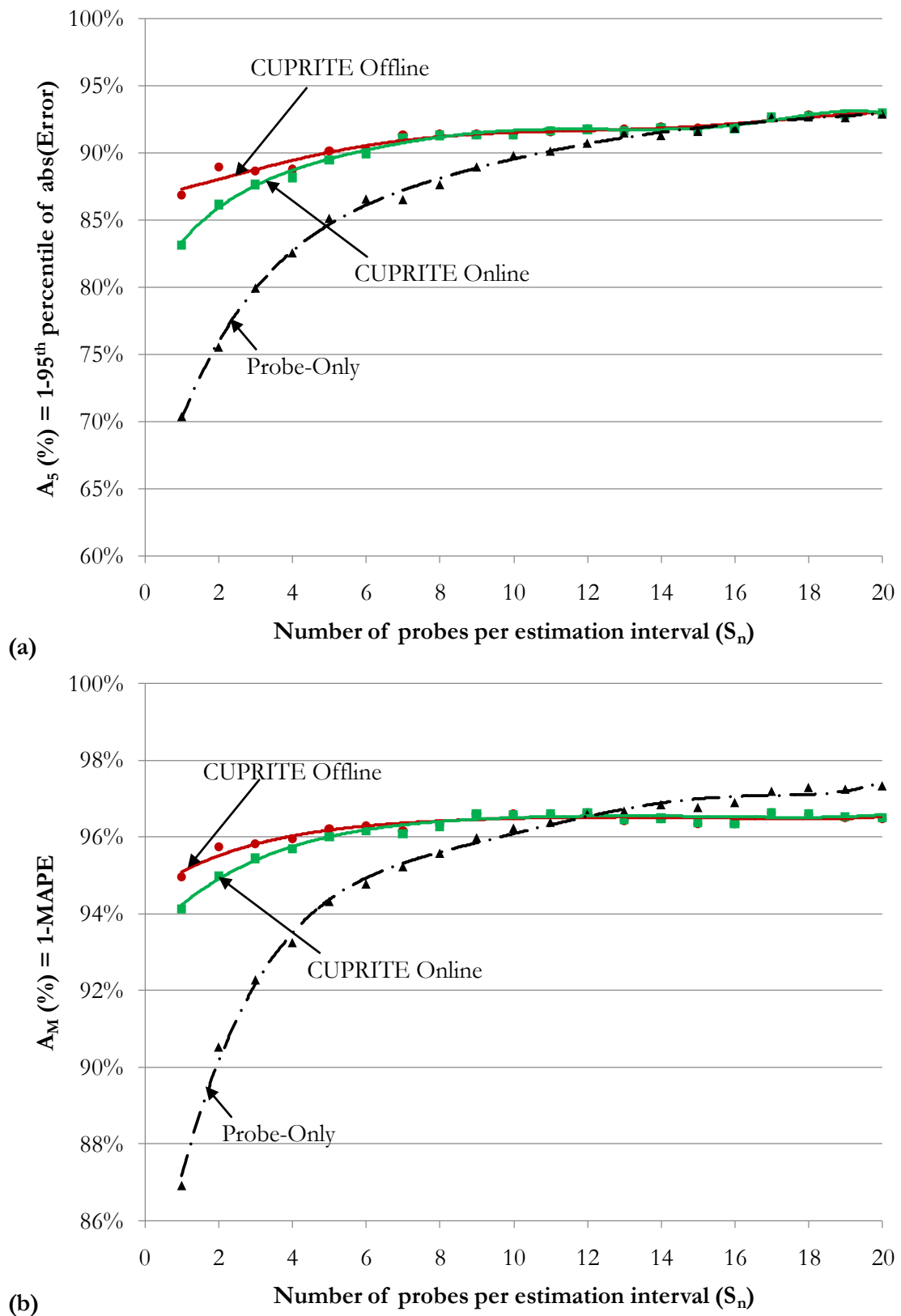
Figure 3-22: Case B1 (10% sink) oversaturated traffic condition for non-FIFO discipline. Results for accuracy: a) A_5 and b) A_M versus S_n .
