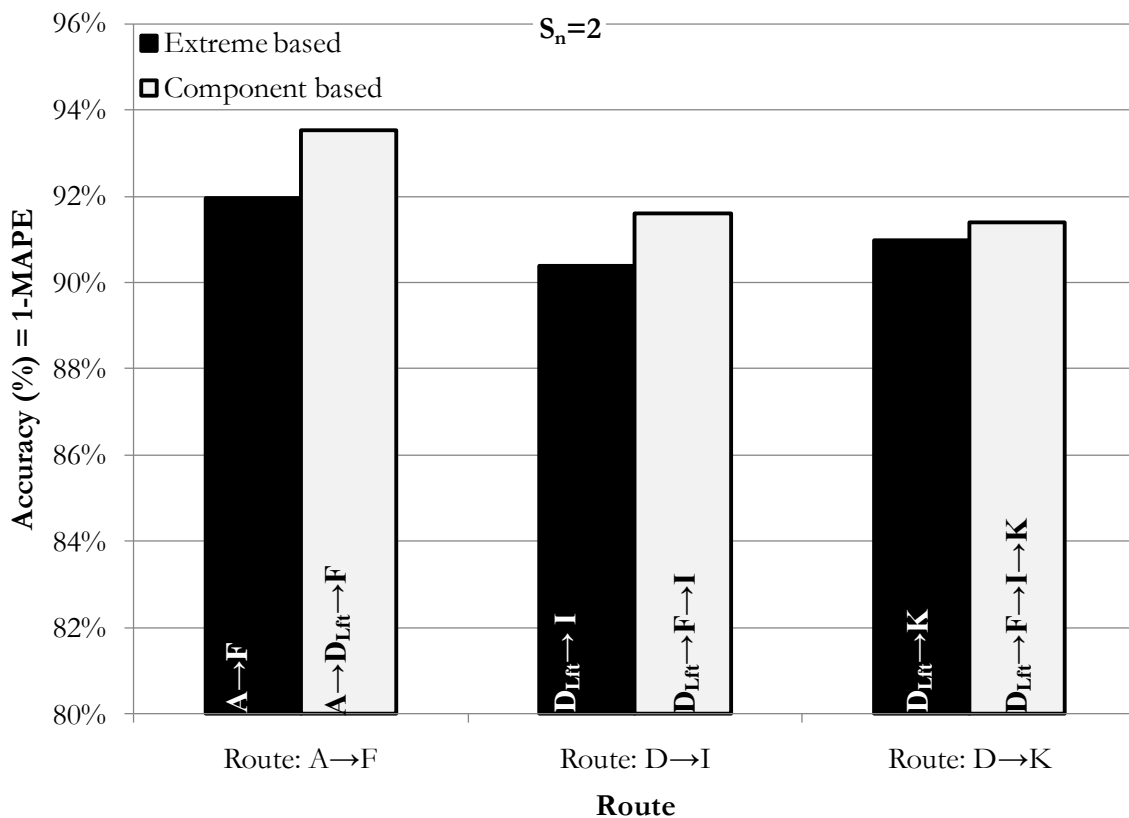
Figure 5-29: Results of Extreme based and Component based travel time estimation for different routes with S_n = 2 .
