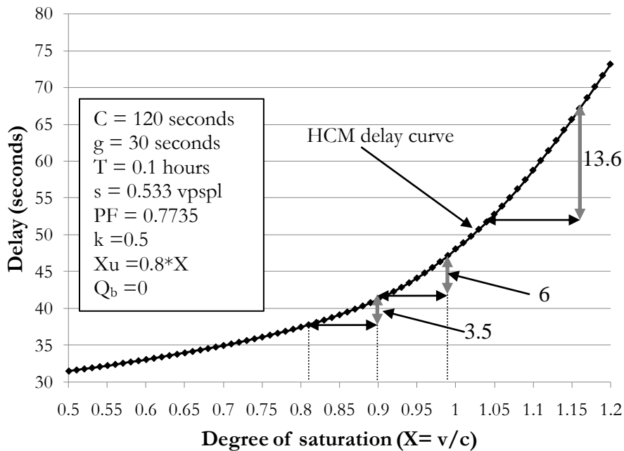
Figure 3-21: HCM 2000 delay versus degree of saturation at downstream intersection.
