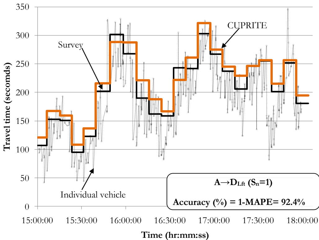
Figure H-3: Q_3 estimation using CUPRITE for route from A → D Lft (S n =1).
