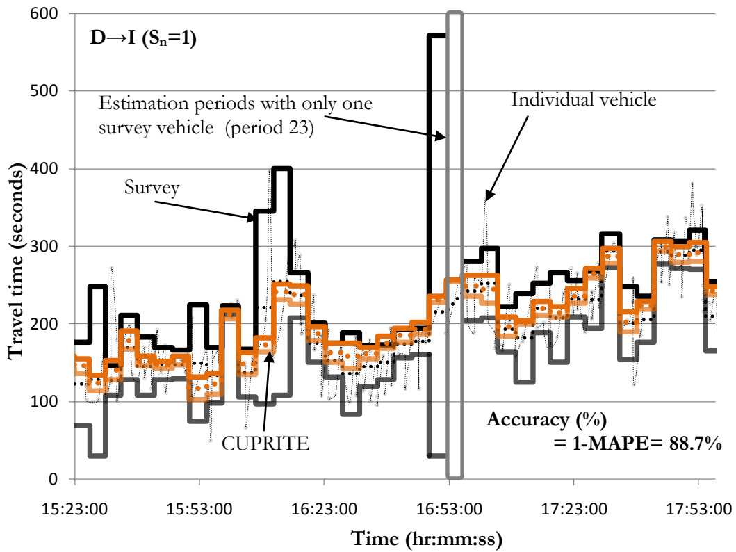
Figure E-2: Extreme based results for D→I ( S_n=1 ).
