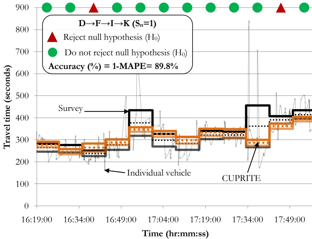
Figure F-4: Component based results for D→F→I→K ( S_n=1 ).
