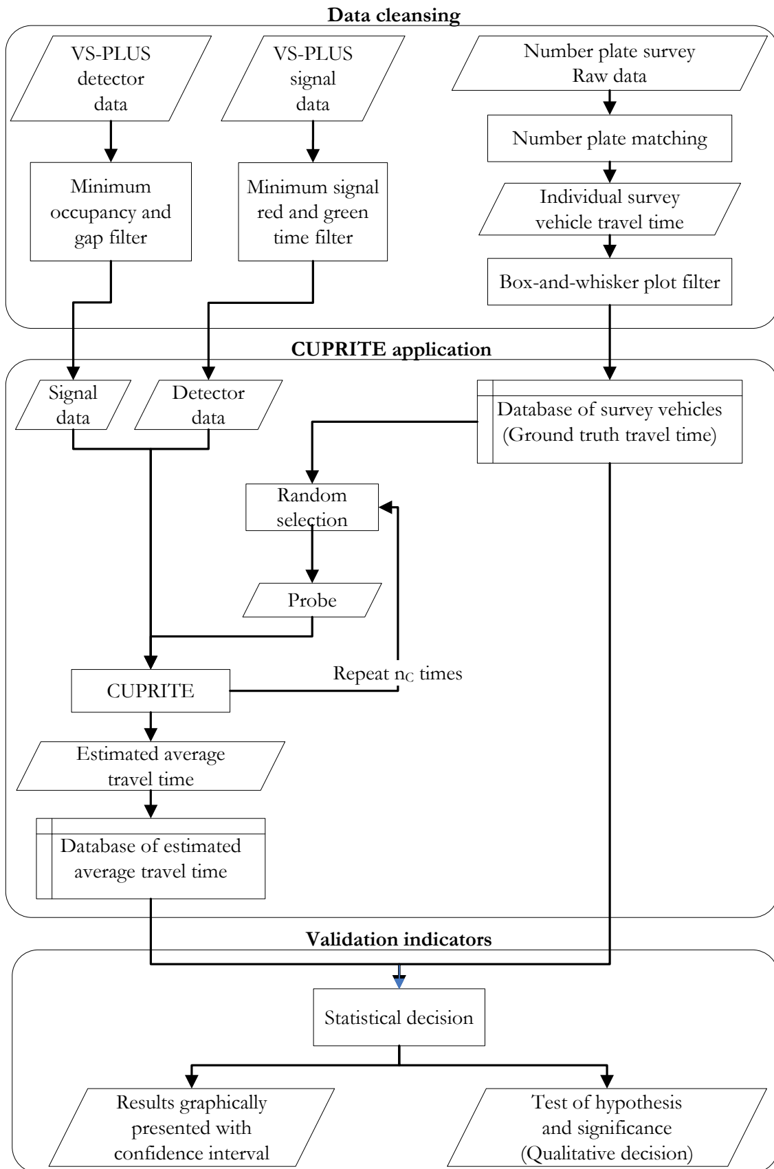
Figure 5-2: Framework for CUPRITE validation.
