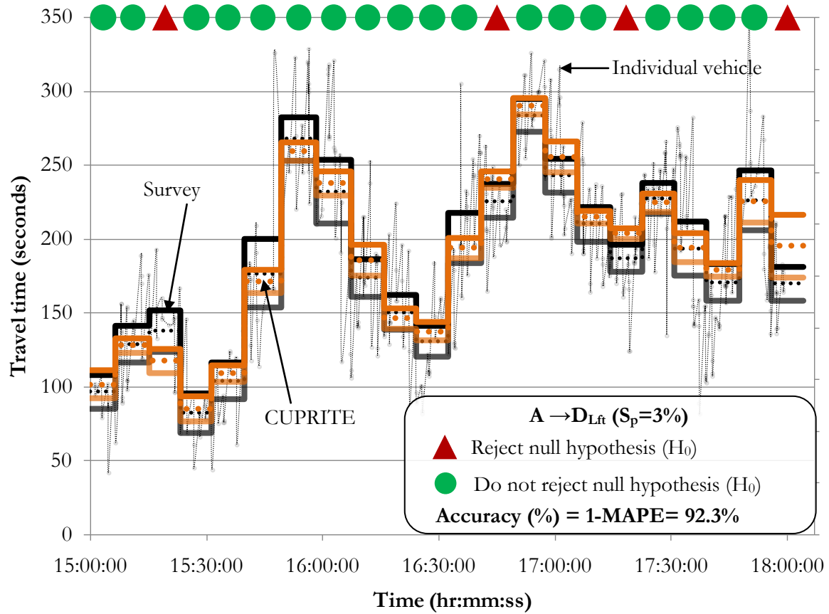
Figure 5-33: Results for A \rightarrow D_{Lft} with S_p=3\% .
