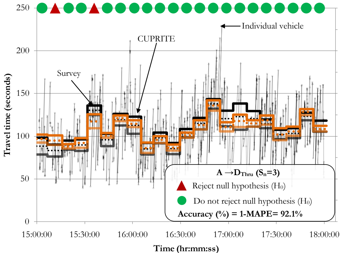
Figure 5-21: Results for A \rightarrow D_{\text{Thru}} with S_n = 3 .
