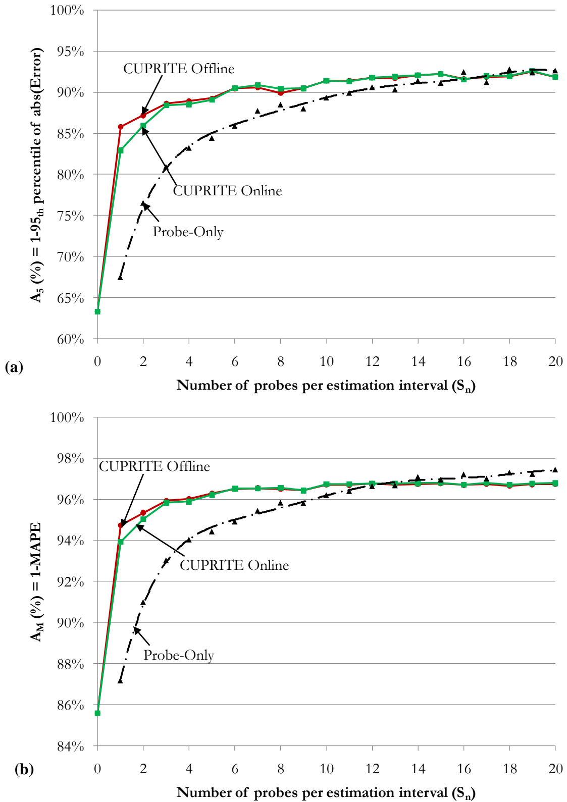
Figure C-18: Results for case B4.8 (10% sink; 10% source; both u/s and d/s detectors overcounting by 10%): (a) A_5 and (b) A_M versus S_n .
