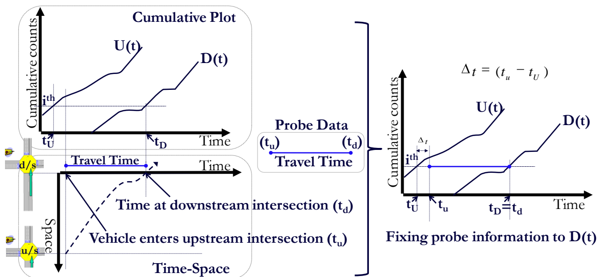
Figure 3-2: Probe vehicle and cumulative plots. Fixing probe information to D(t) .
