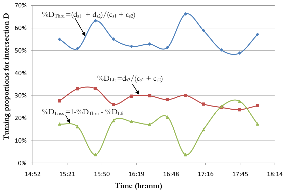
Figure 5-13: Turning proportions for different directions from C to D .
