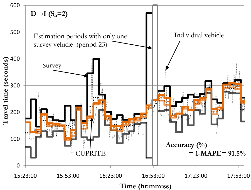
Figure E-3: Extreme based results for D→I ( S_n=2 ).
