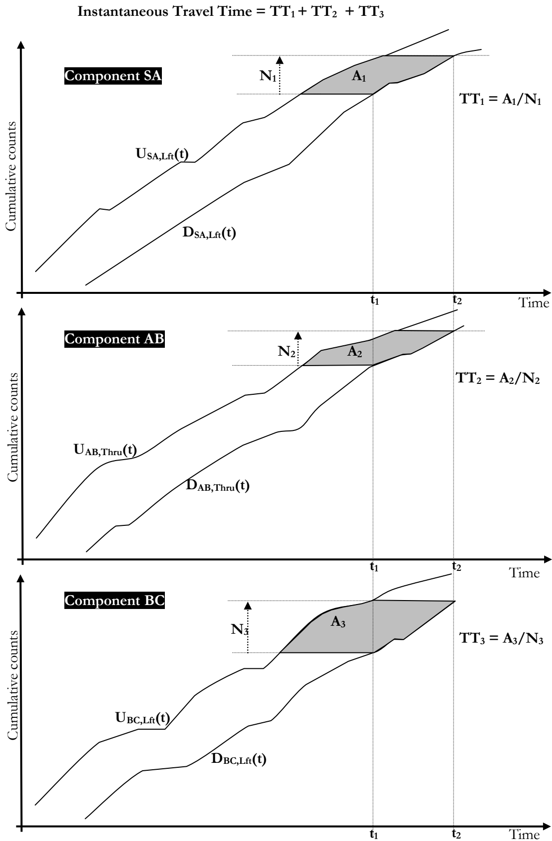
Figure 4-9: Example for instantaneous route travel time.
