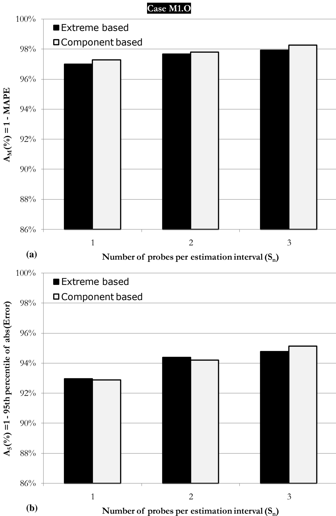
Figure 4-14: Case Study M1.O, Flow = F1, Accuracy (a) A_M and (b) A_5 versus S_n .
