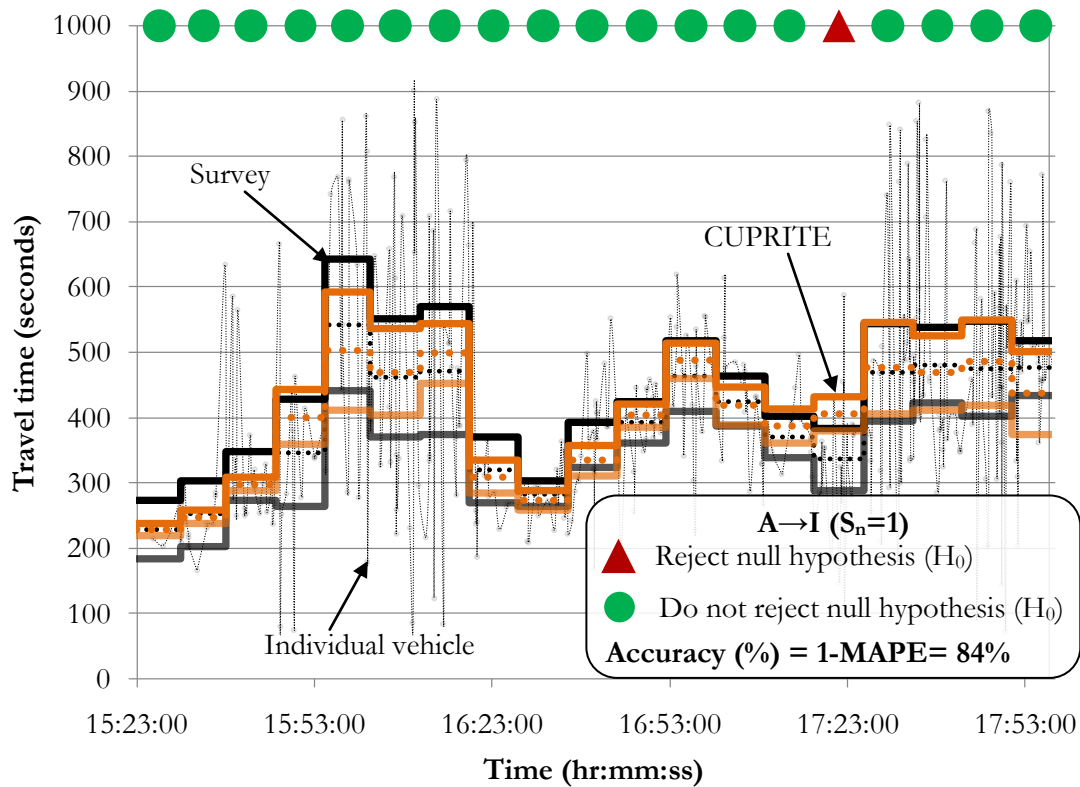
Figure G-1: Extreme based results for A→I (S n =1).
