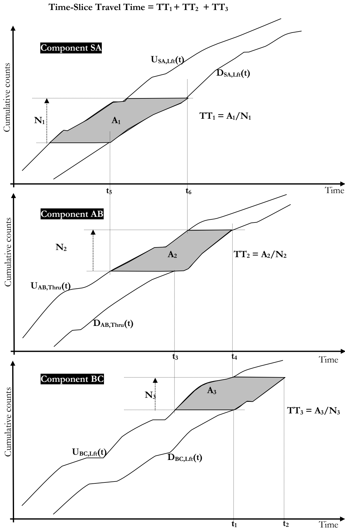
Figure 4-10: Example for time-slice route travel time: Component based (R C ) .
