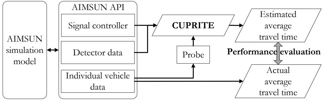
Figure 3-11: Architecture for CUPRITE testing using AIMSUN.
