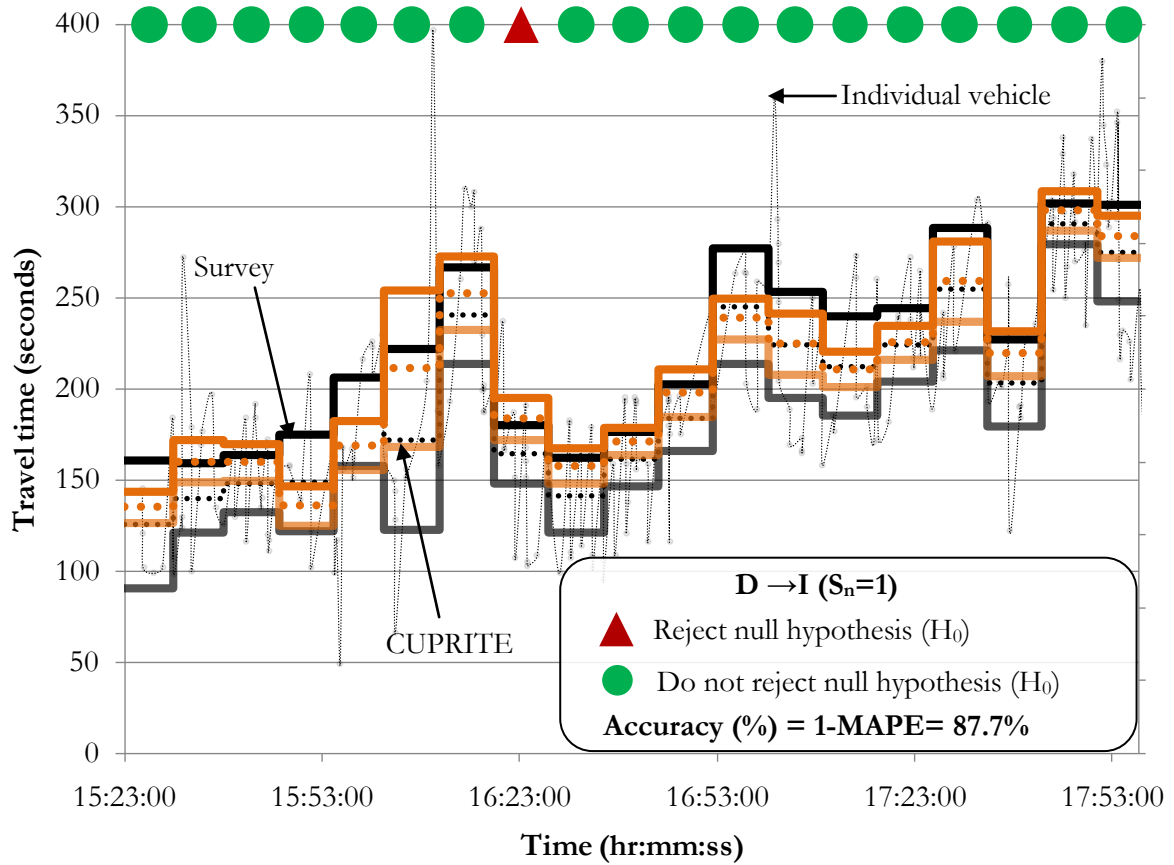
Figure 5-22: Results for D→I with S_n = 1 .
