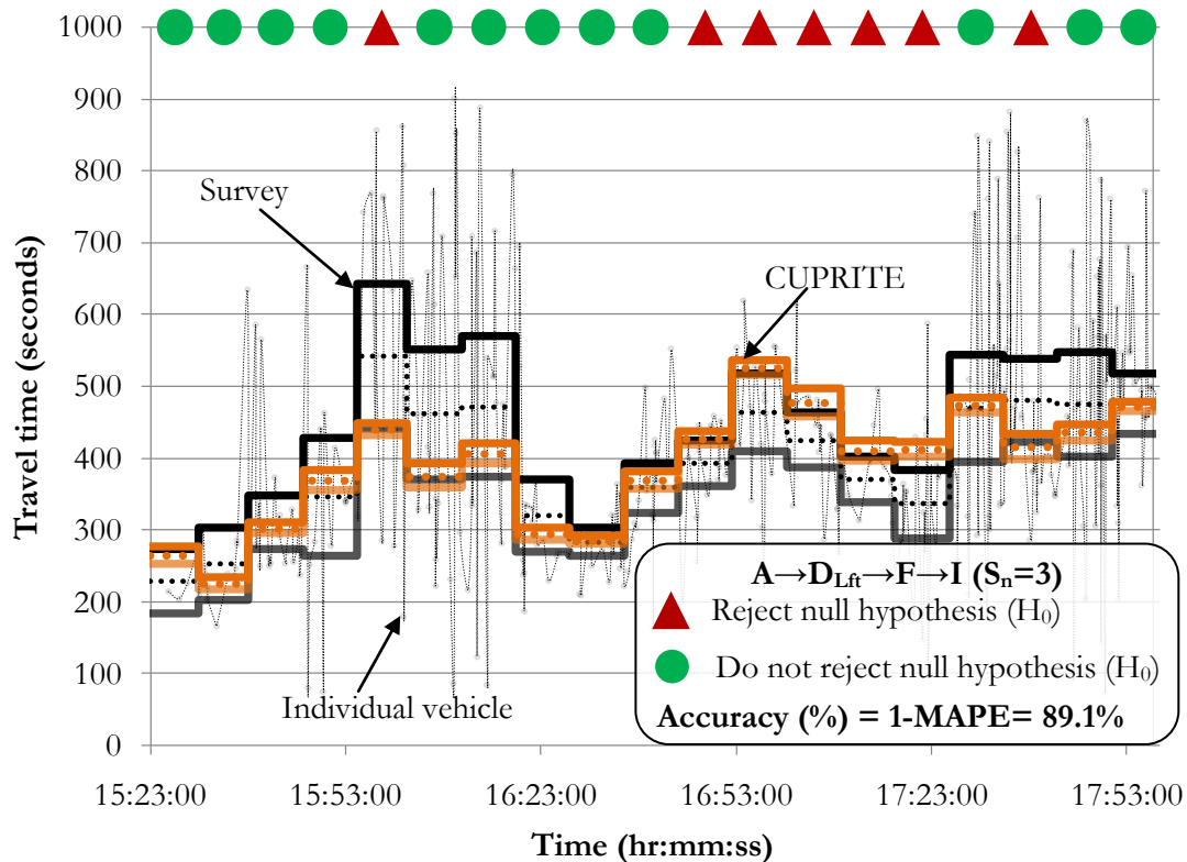
Figure G-6: Component based results for A \rightarrow D_{Lft} \rightarrow F \rightarrow I (S_n=3) .
