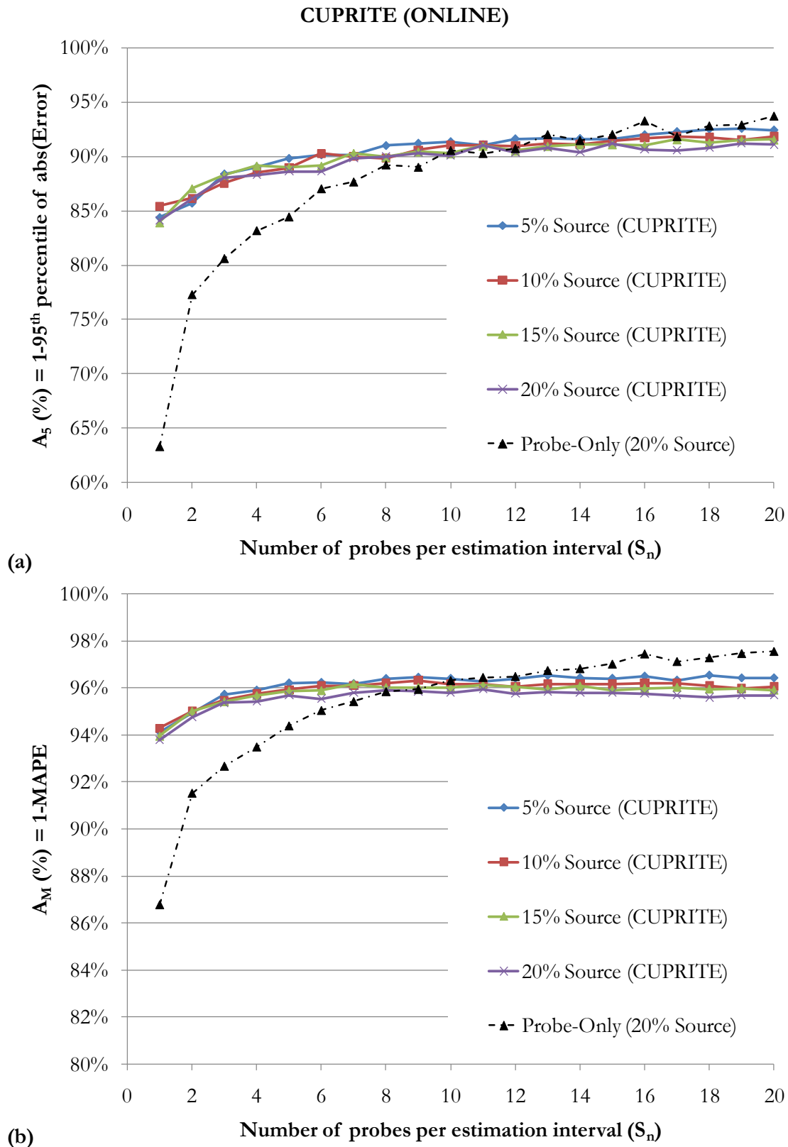
Figure C-7: CUPRITE Online application for different source percentages (5%, 10%, 15% and 20%); oversaturated traffic condition; non-FIFO discipline. Results for accuracy: (a) A_5 and (b) A_M versus S_n .
