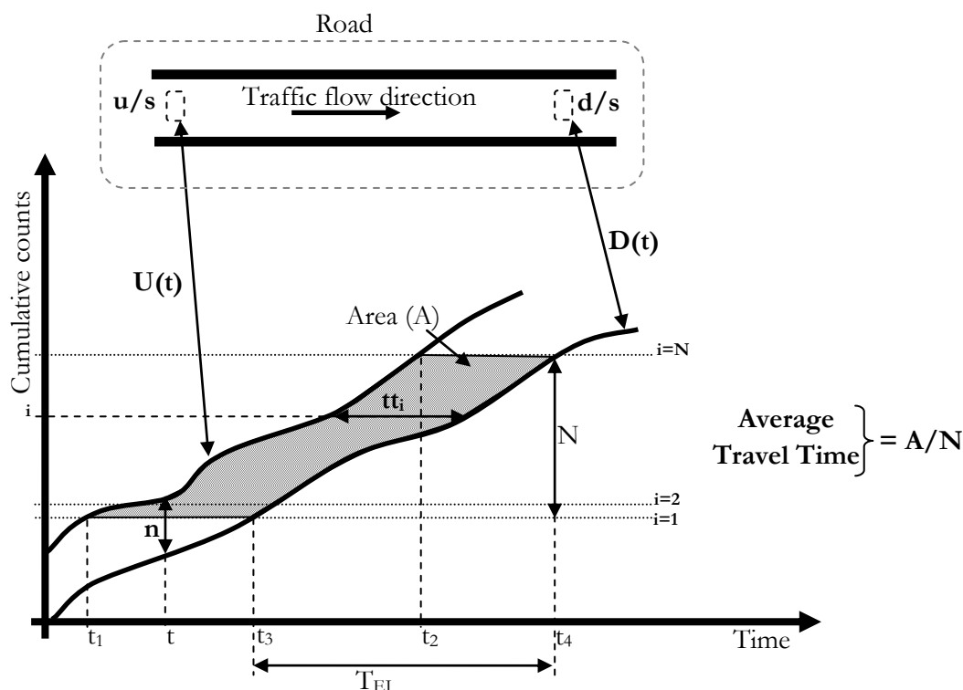
Figure 1-2: Classical analytical procedure for average travel time estimation.
