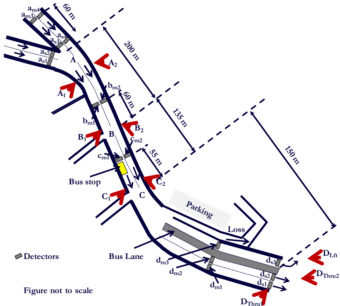
Figure 5-12: Illustration of the link characteristics between intersections A and D .
