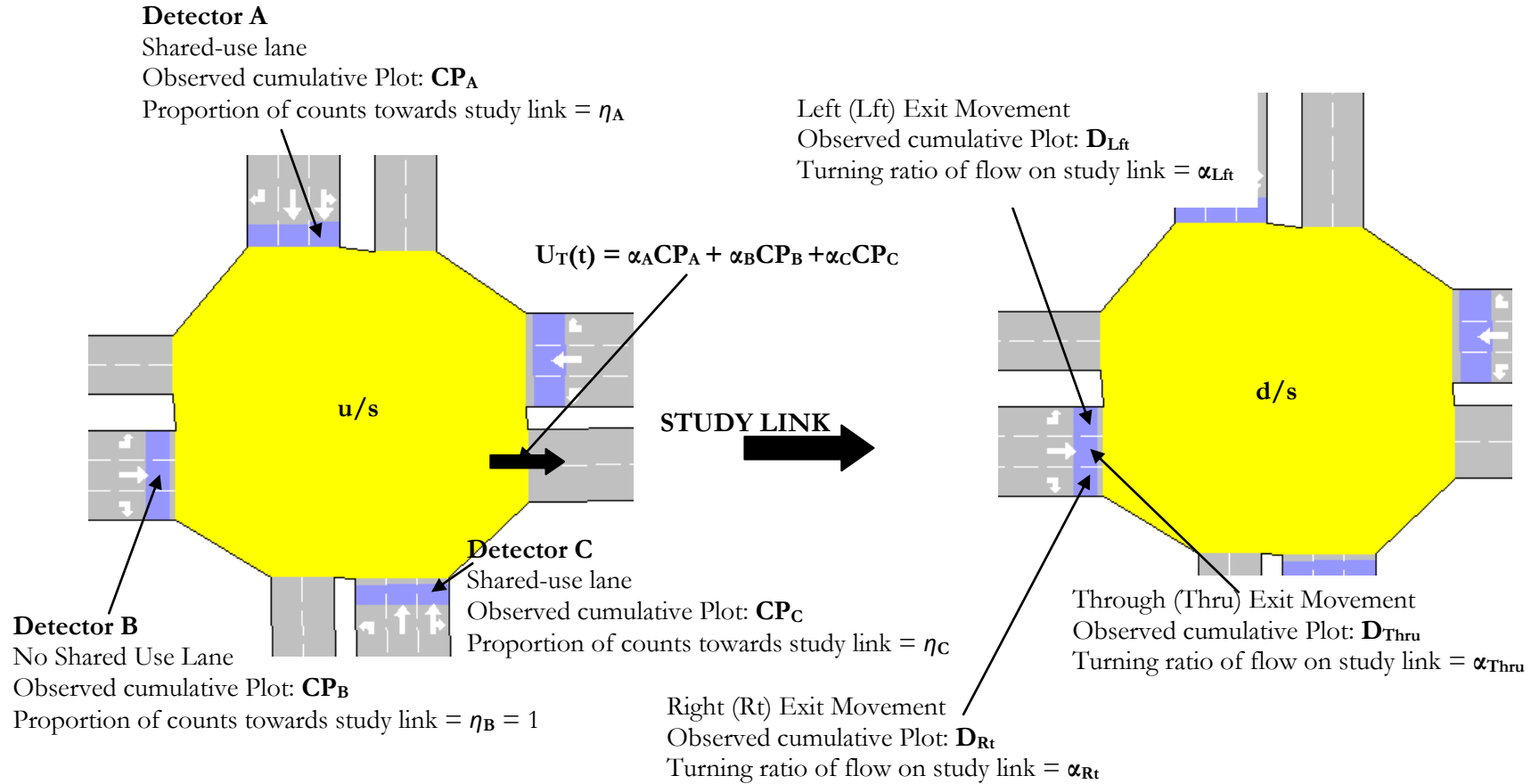
Figure 4-4: Example of a study link with flow from three different directions at upstream intersection and exit flow towards three different movements at downstream intersection.
