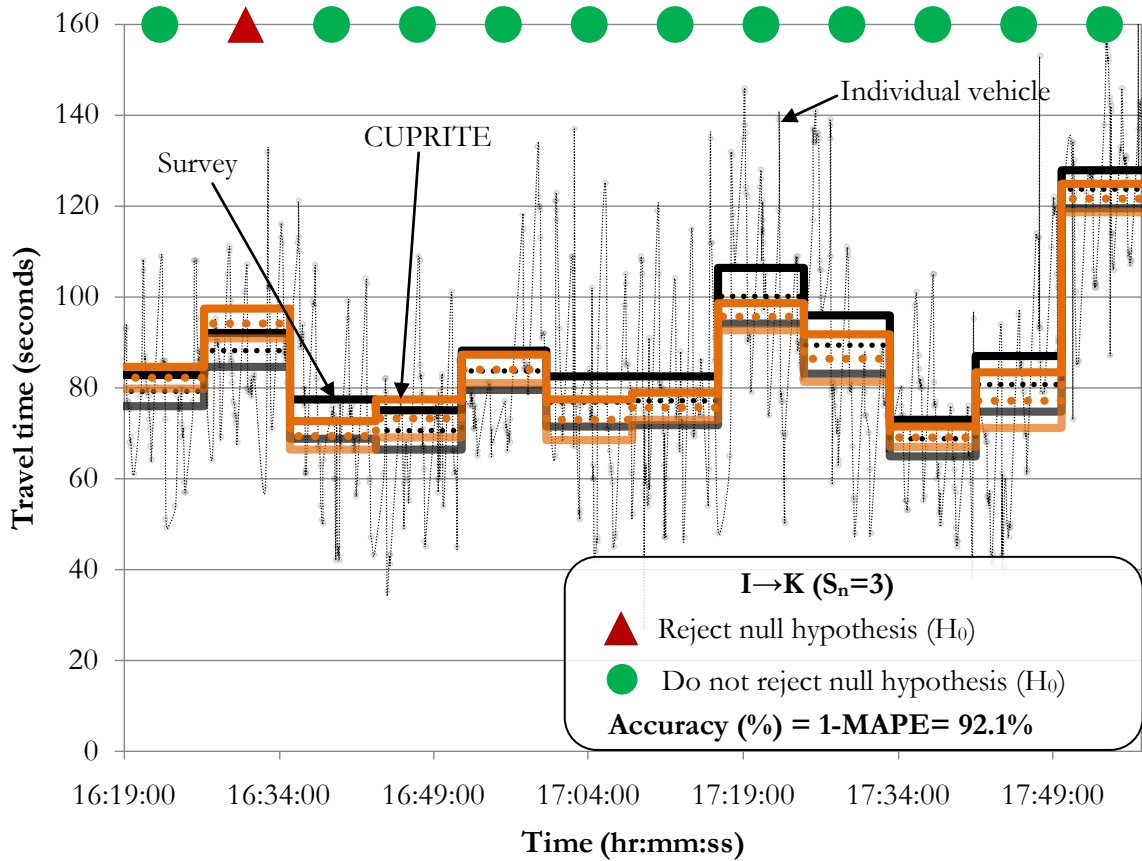
Figure 5-27: Results for I→K with S_n = 3 .
