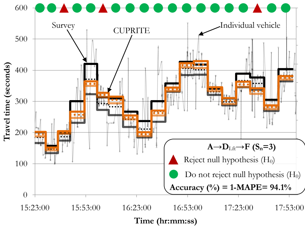
Figure D-6: Component based results for A \rightarrow D_{Lft} \rightarrow F (S_n=3) .
