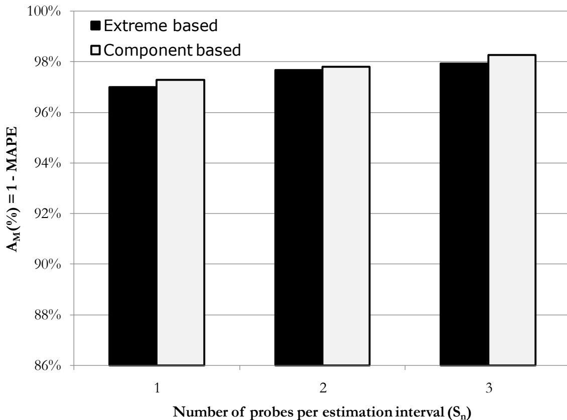
Figure 0-3: Comparative overview of Accuracy ( A_M ) from Component based and Extreme based versus S_n .
