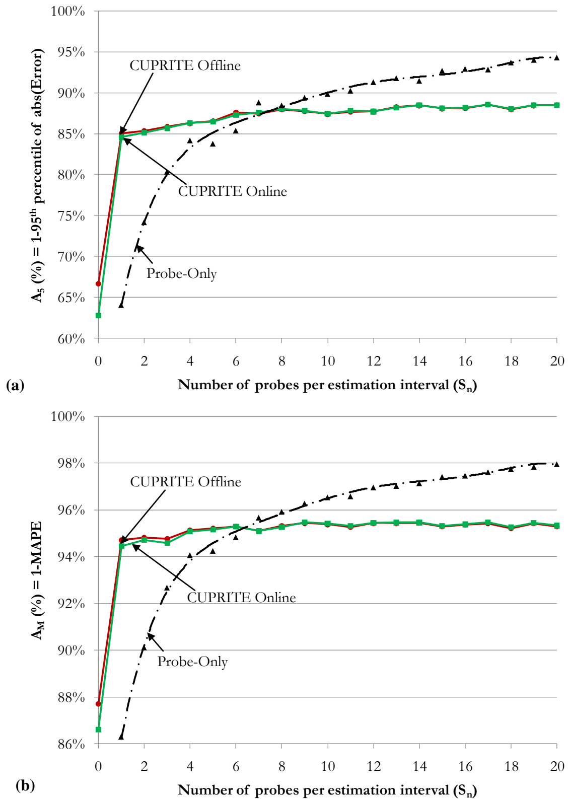
Figure C-15: Simultaneous presence of both sink and source. Case B4.5 (50% sink and 50% source): (a) A_5 and (b) A_M versus S_n .
