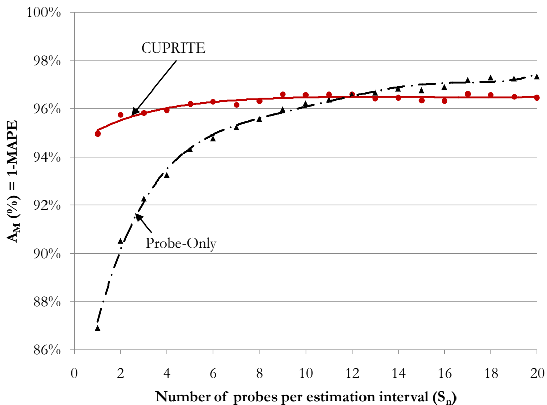
Figure 0-1: Comparative results for accuracy: versus fixed number of probes per estimation period for CUPRITE and Probe-Only method.
