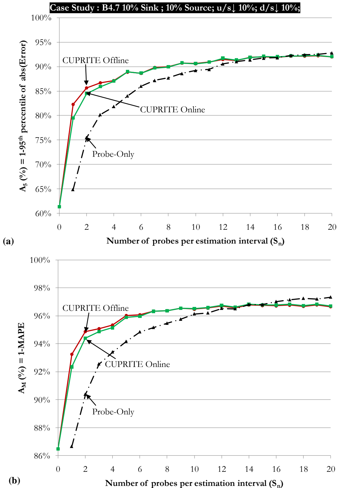
Figure C-17: Simultaneous presence of sink, source and detector counting error. Case B4.7 (10% sink; 10% source; both u/s and d/s detectors undercounting by 10%): (a) A_5 and (b) A_M versus S_n .
