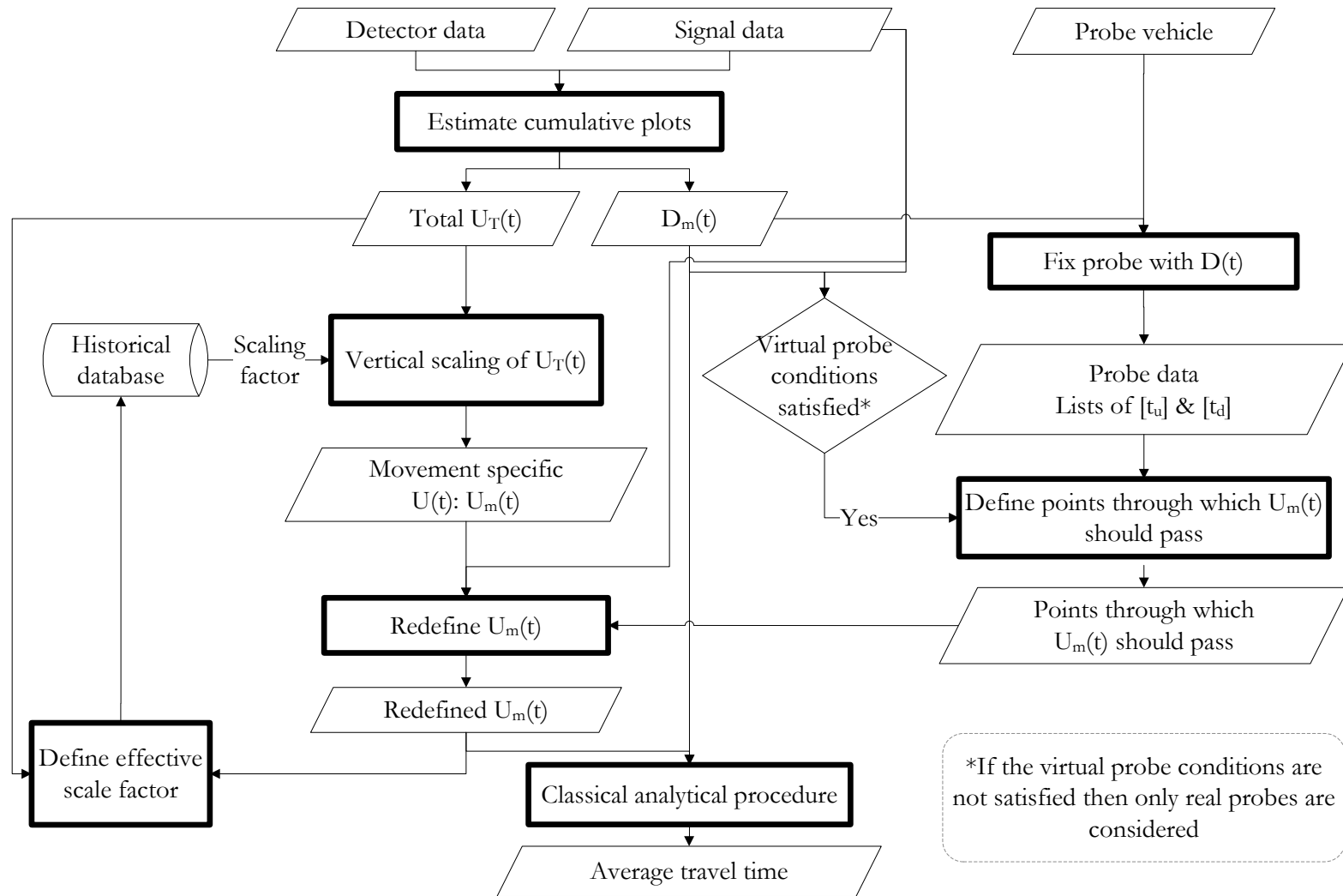
Figure 4-7: CUPRITE architecture for link-movement specific travel time estimation.
