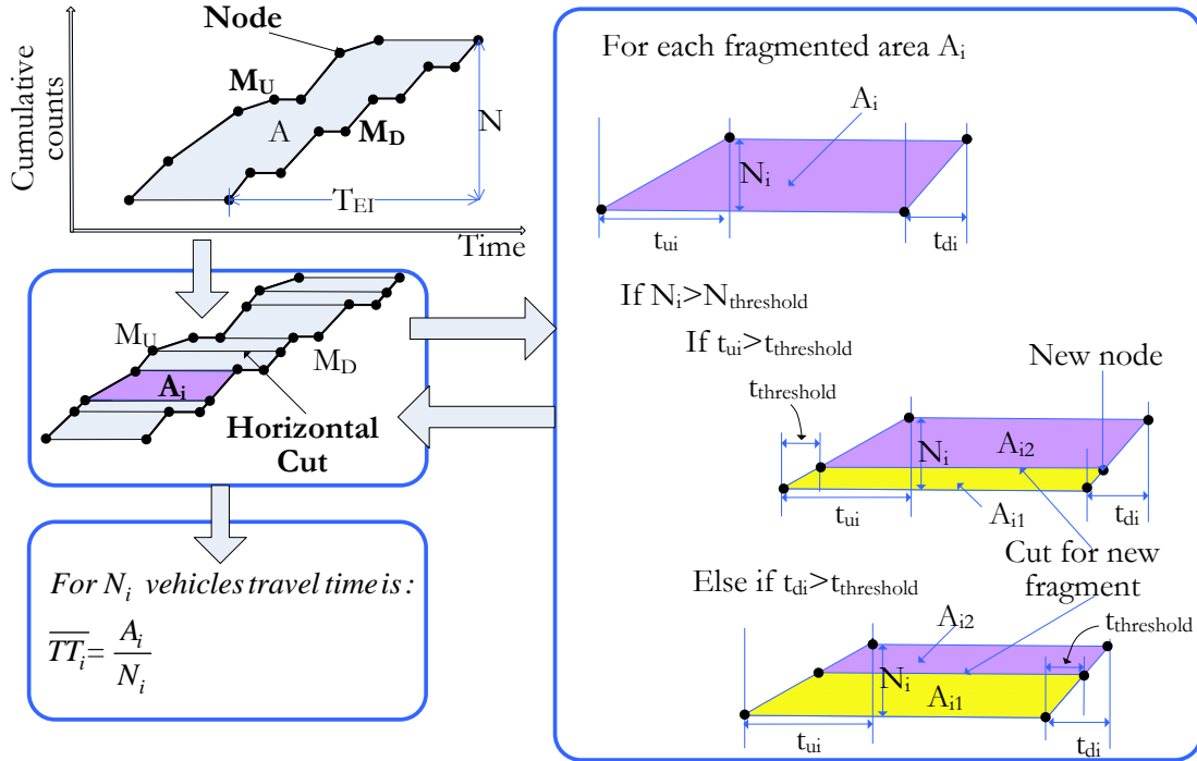
Figure H-1: Illustration for slicing the area between cumulative plots for defining travel time for different pair of vehicles within a estimation interval.
