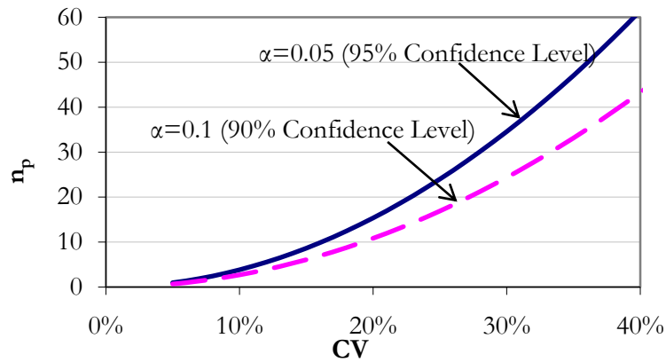
Figure 2-1: Relation between number of probes and coefficient of variation for 95% and 90% confidence level and 10 % error.
