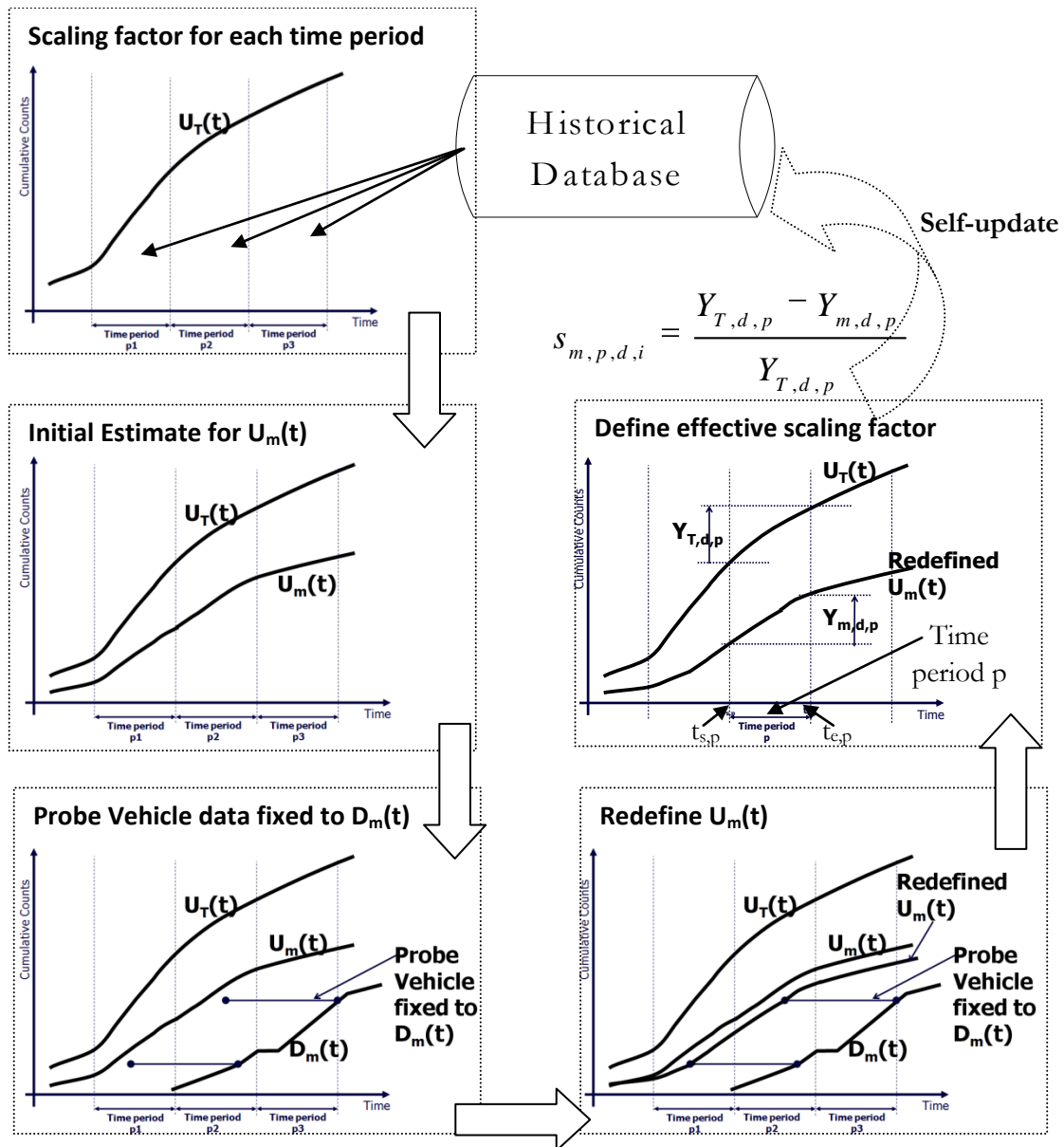
Figure 4-6: Example of the methodology for estimation of upstream cumulative plot for each exit turning movement.
