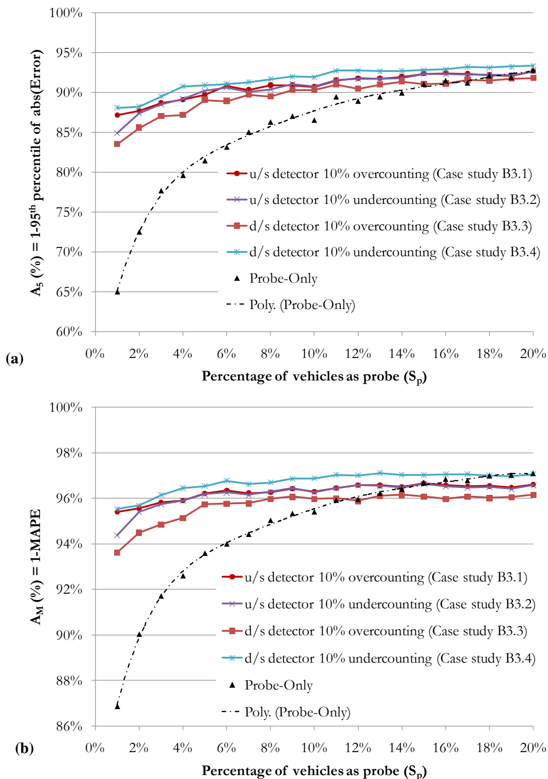
Figure C-11: Results for accuracy versus S_p case B3.1 to case B3.4 from CUPRITE offline application.
