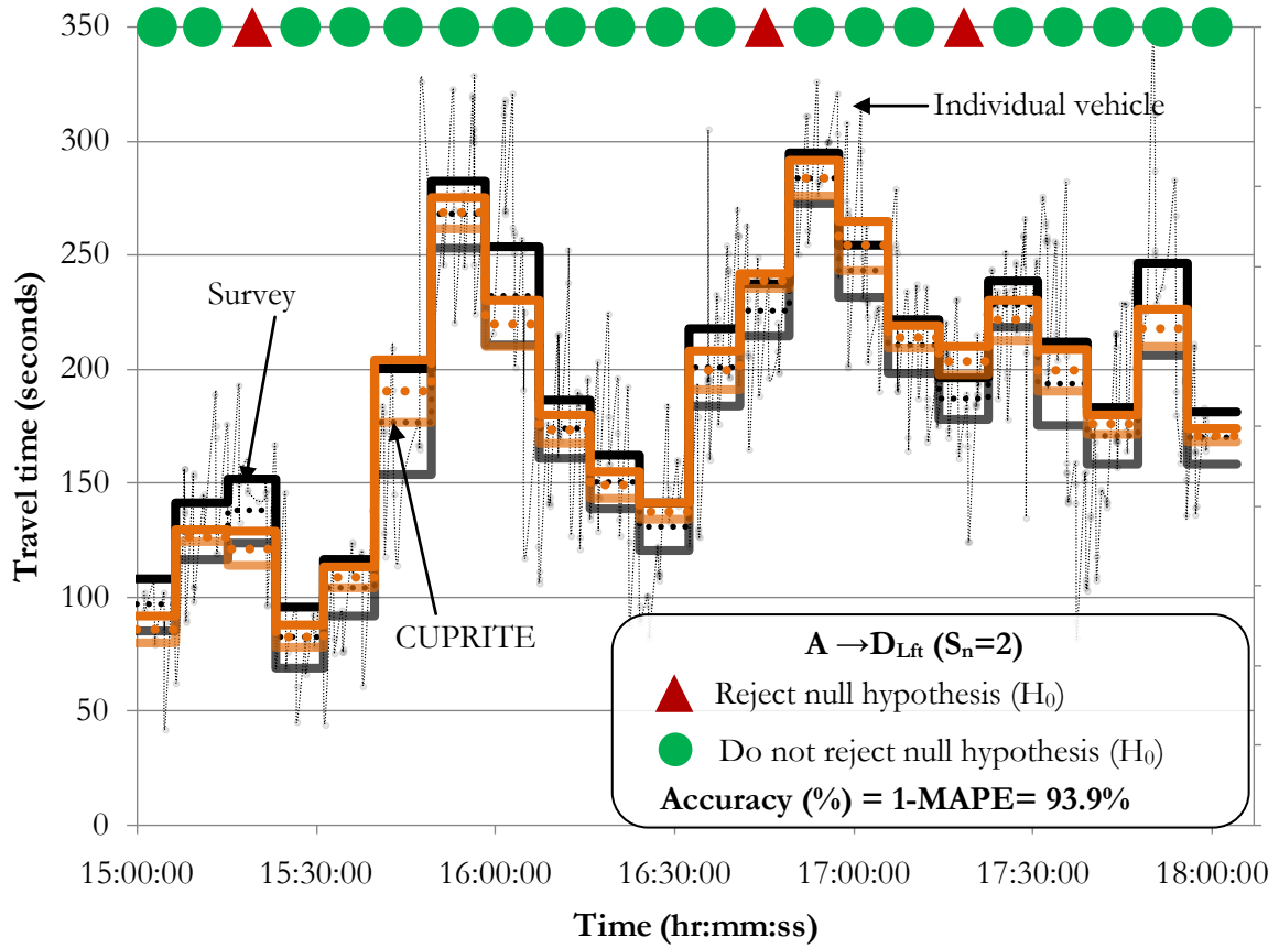
Figure 5-17: Results for A \rightarrow D_{Lft} with S_n = 2 .
