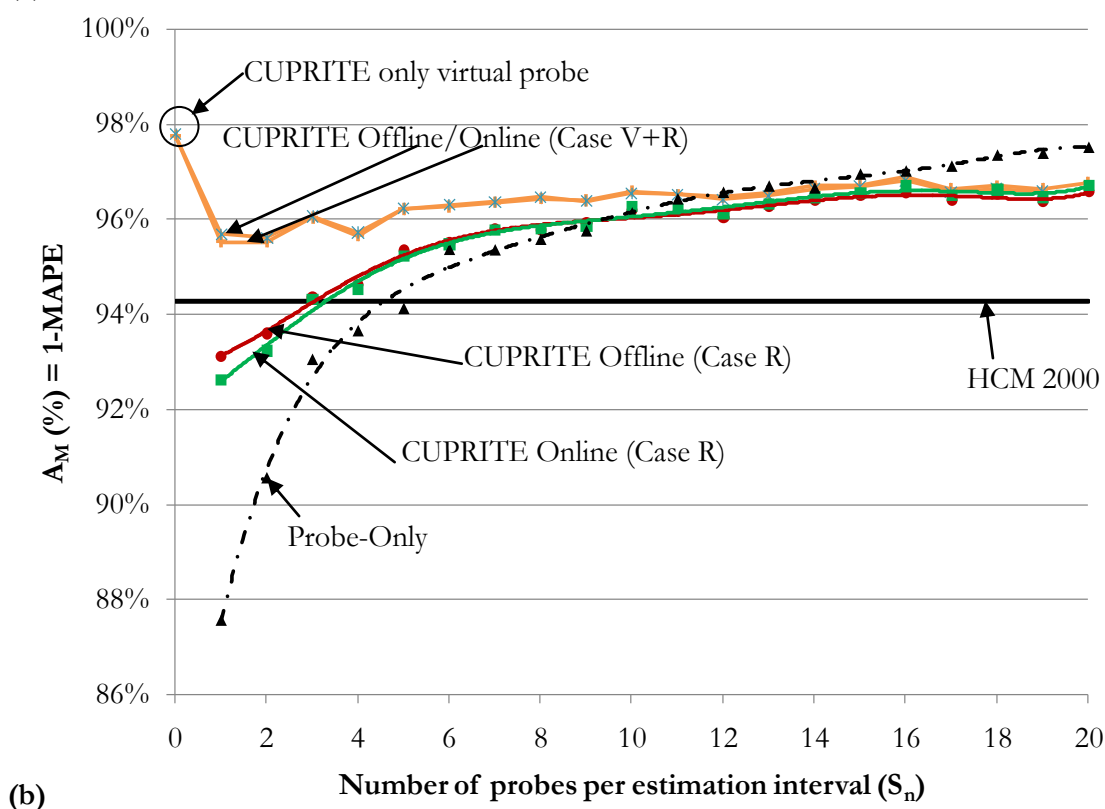
Figure 3-17: Comparative results for 10% downstream detector overcounting case during undersaturated traffic condition. Results for accuracy : (a) A_5 and (b) A_M .
