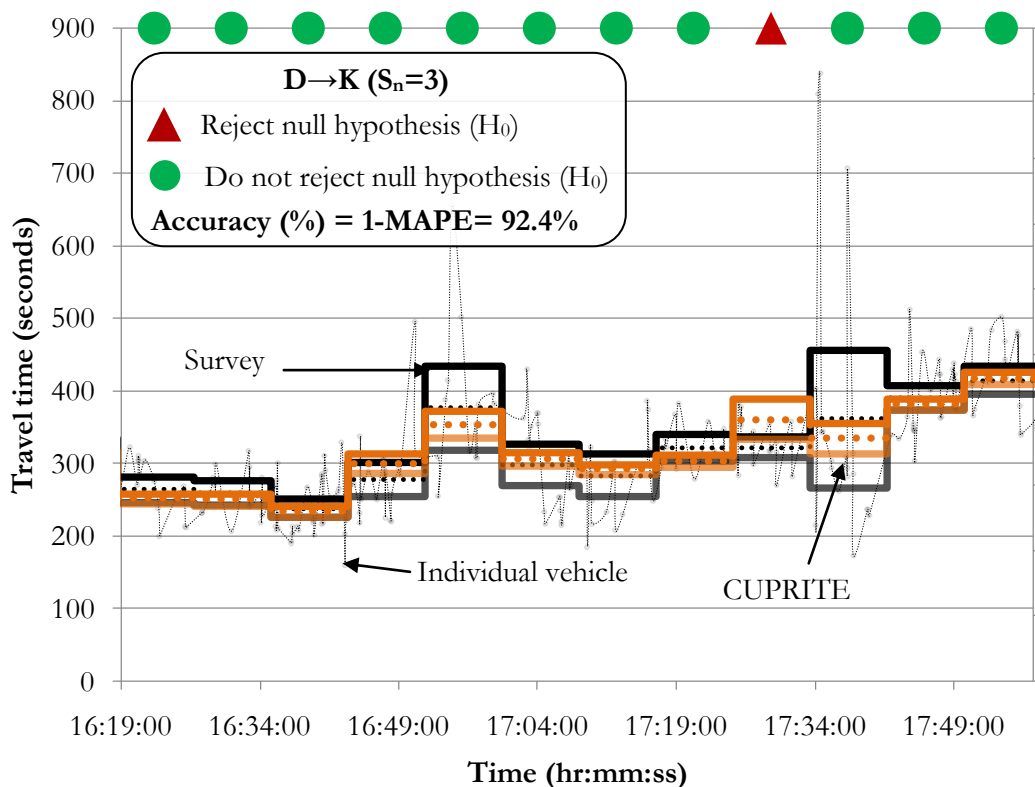
Figure F-3: Extreme based results for D→K ( S_n=3 ).
