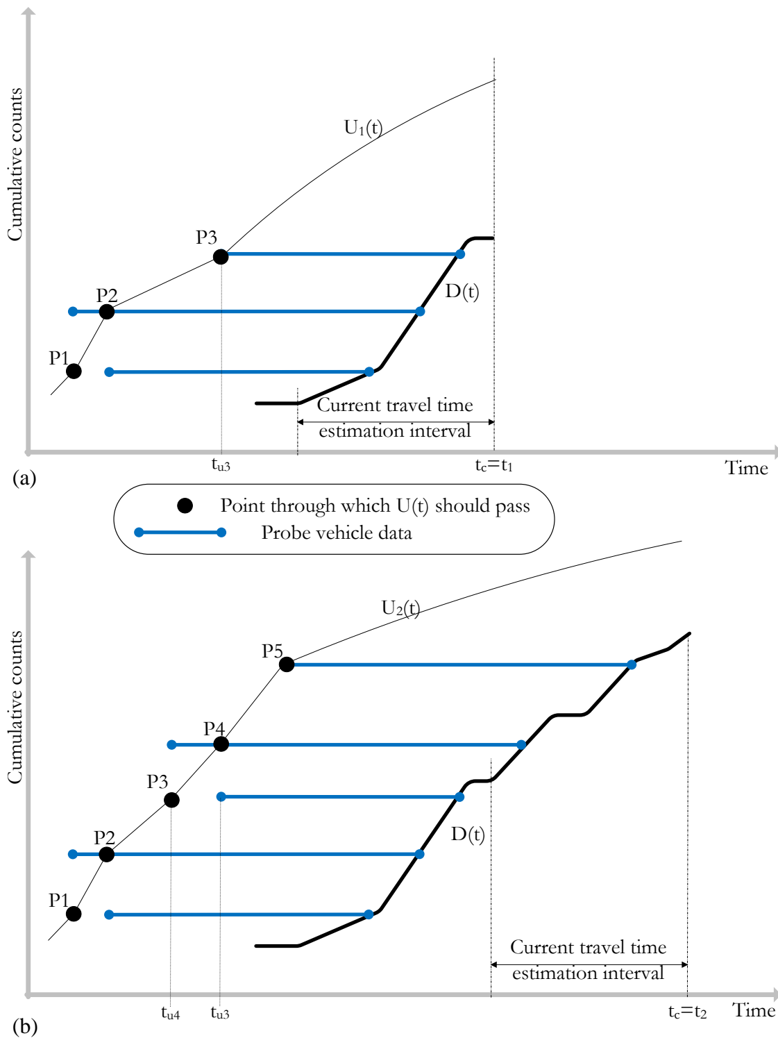
Figure 3-9: Example for defining the points from where the U(t) should pass for online application: a) at time t_1 ; b) at time t_2 .
