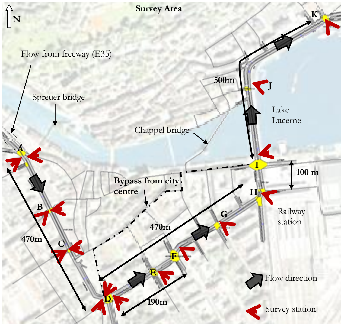
Figure 5-11: Number plate survey stations.
