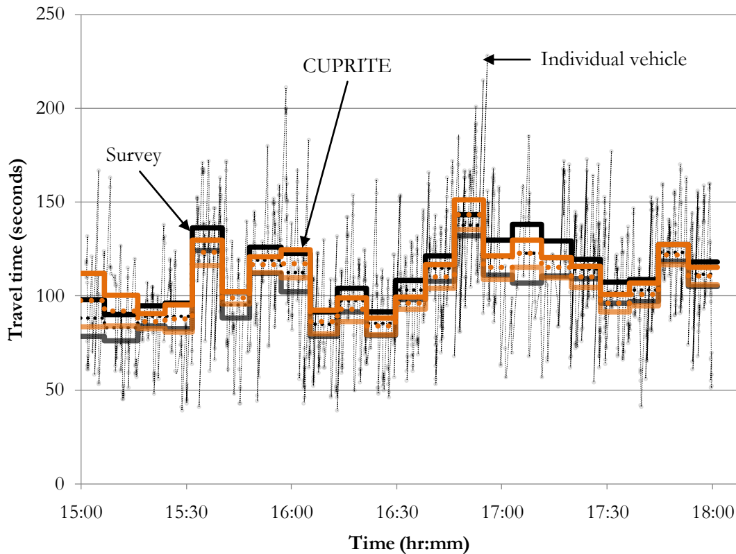
Figure 0-5: Results for A \rightarrow D_{\text{Thru}} with S_n = 2 .
