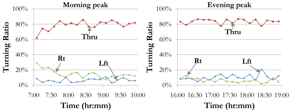
Figure 4-5: Example for real turning ratios for three different directions from one of the link at Ikegami Shinmachi intersection, in Kawasaki City, Japan.
