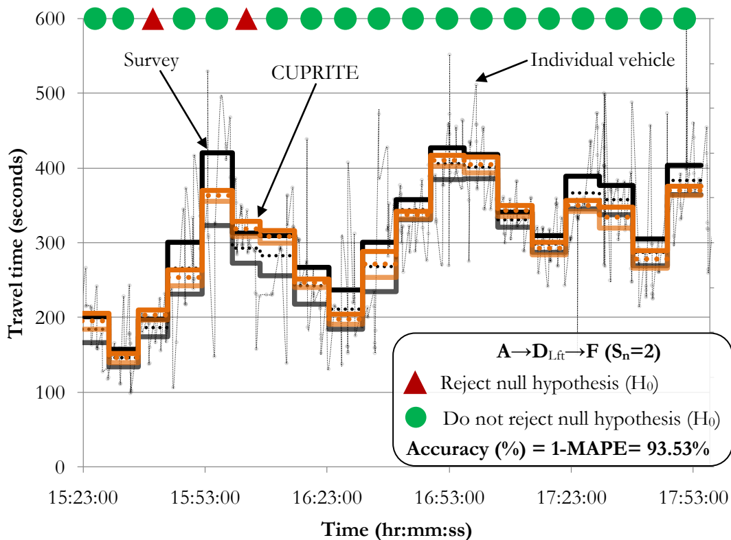
Figure D-5: Component based results for A→D Lft →F (S n =2).
