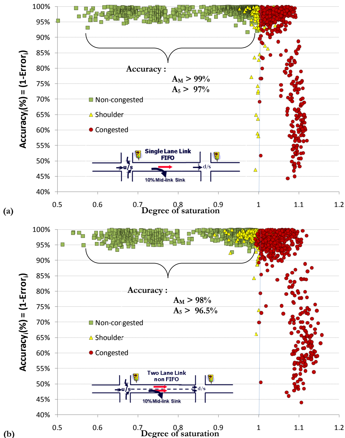
Figure 3-15: Simulation for different traffic flow conditions with no real probe: a) FIFO network and b) non-FIFO network. (Case A1).
