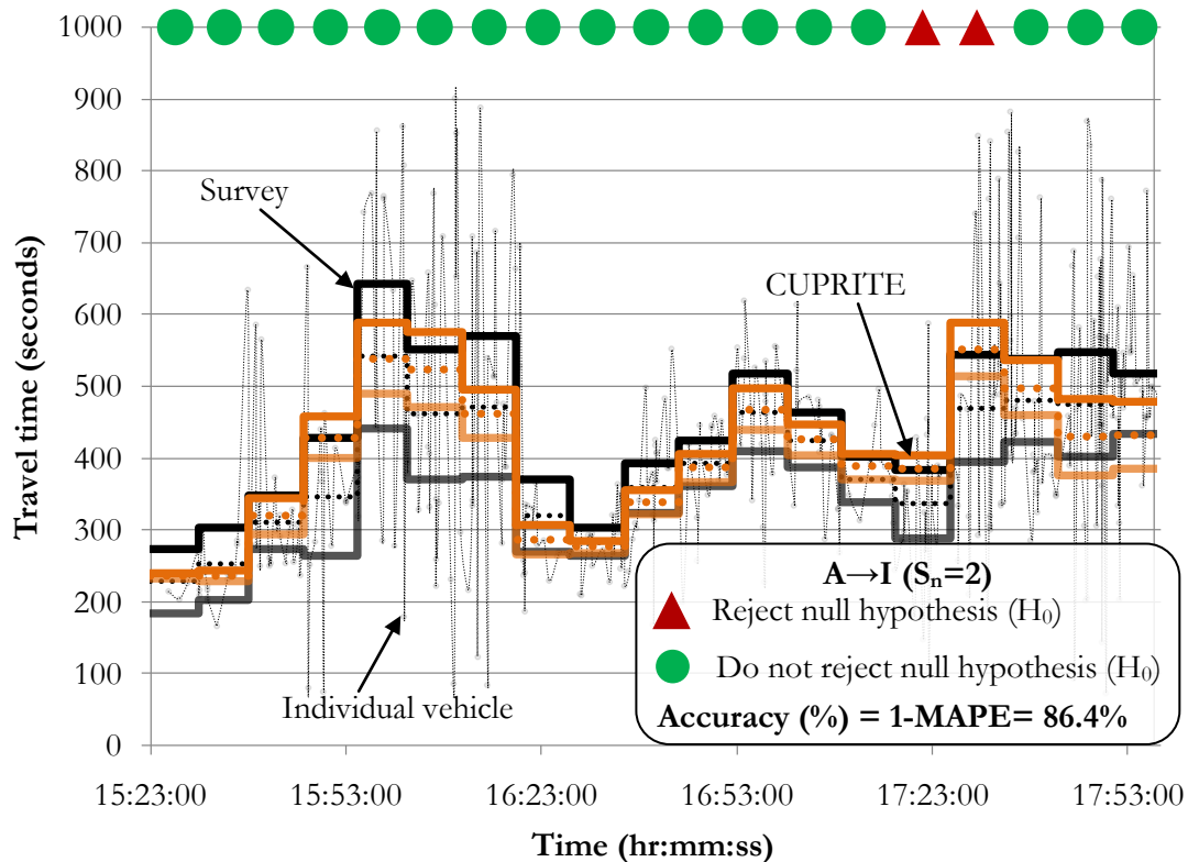
Figure G-2: Extreme based results for A→I ( S_n=2 ).
