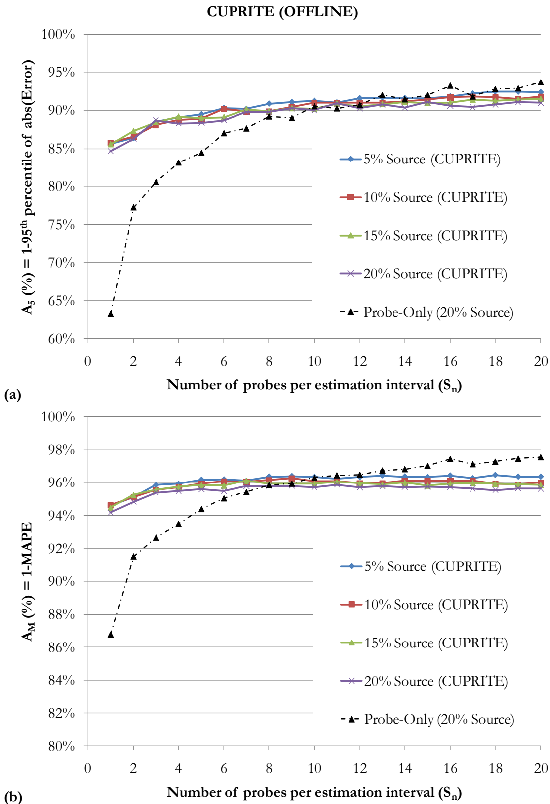
Figure C-6: CUPRITE Offline application for different source percentages (5%, 10%, 15% and 20%); oversaturated traffic condition; non-FIFO discipline. Results for accuracy: (a) A_5 and (b) A_M versus S_n .
