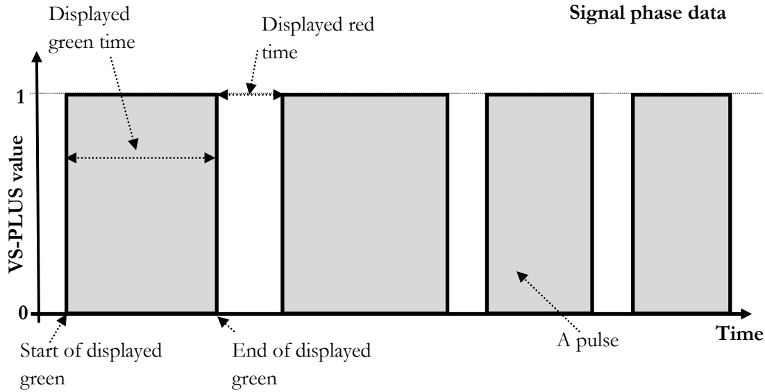
Figure 5-8: Pulse data representation for VS-PLUS signal data.
