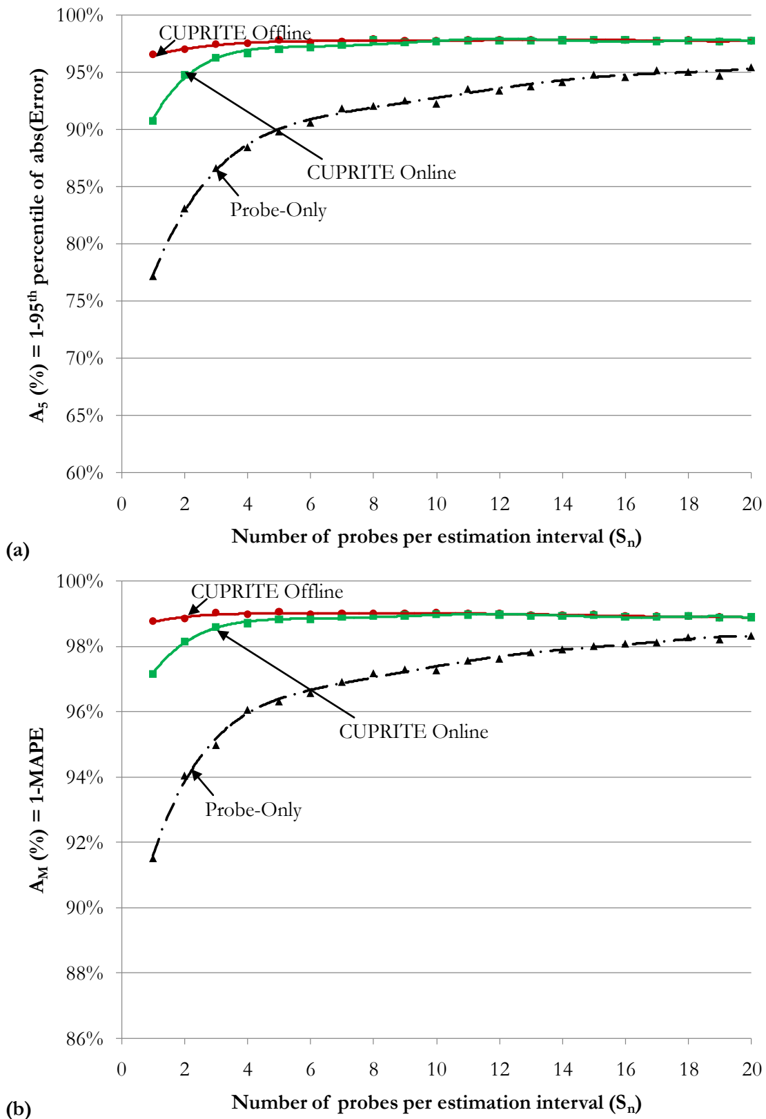
Figure C-5: Case B1 (10% sink) oversaturated traffic condition for FIFO discipline. Results for accuracy: (a) A_5 and (b) A_M versus S_n .
