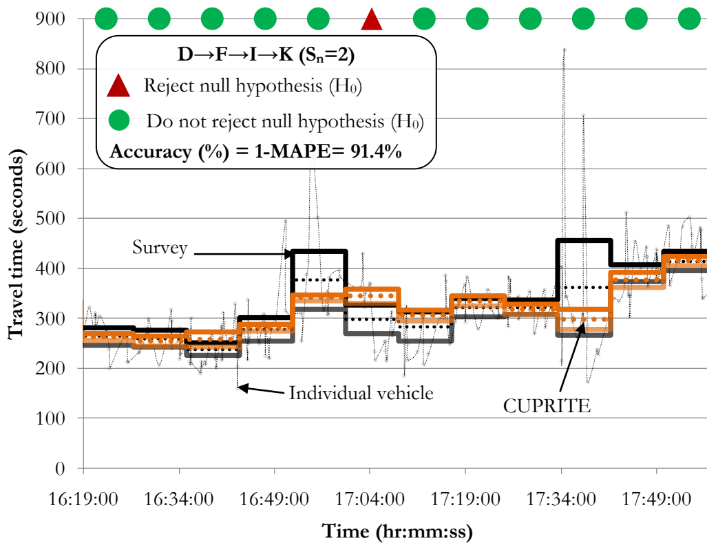
Figure F-5: Component based results for D→F→I→K ( S_n=2 ).
