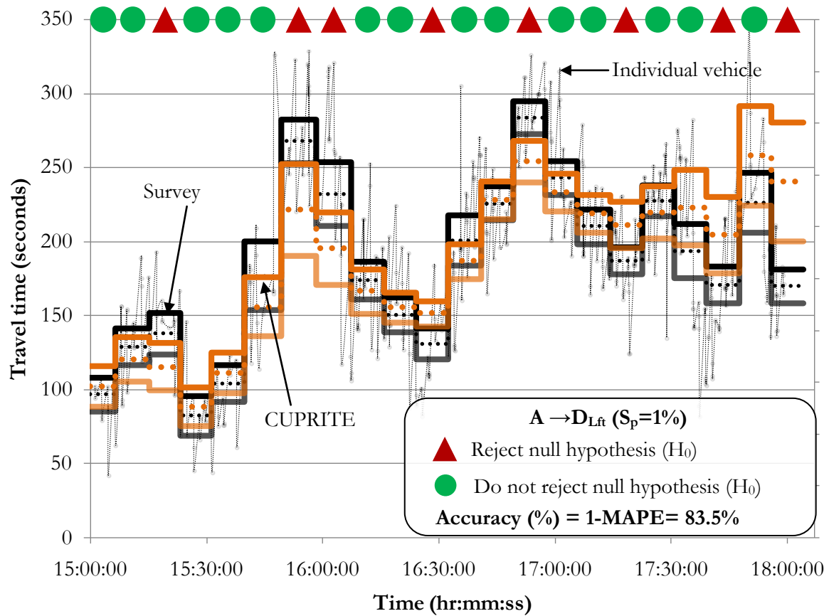
Figure 5-31: Results for A→D Lft with S_p=1\% .
