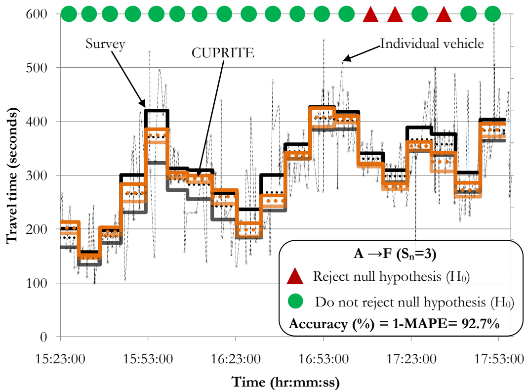
Figure D-3: Extreme based results for A → F ( S_n=3 ).
