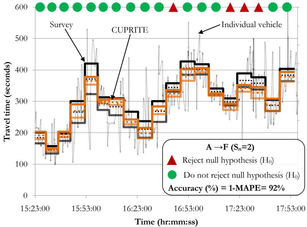
Figure D-2: Extreme based results for A → F ( S_n=2 ).
