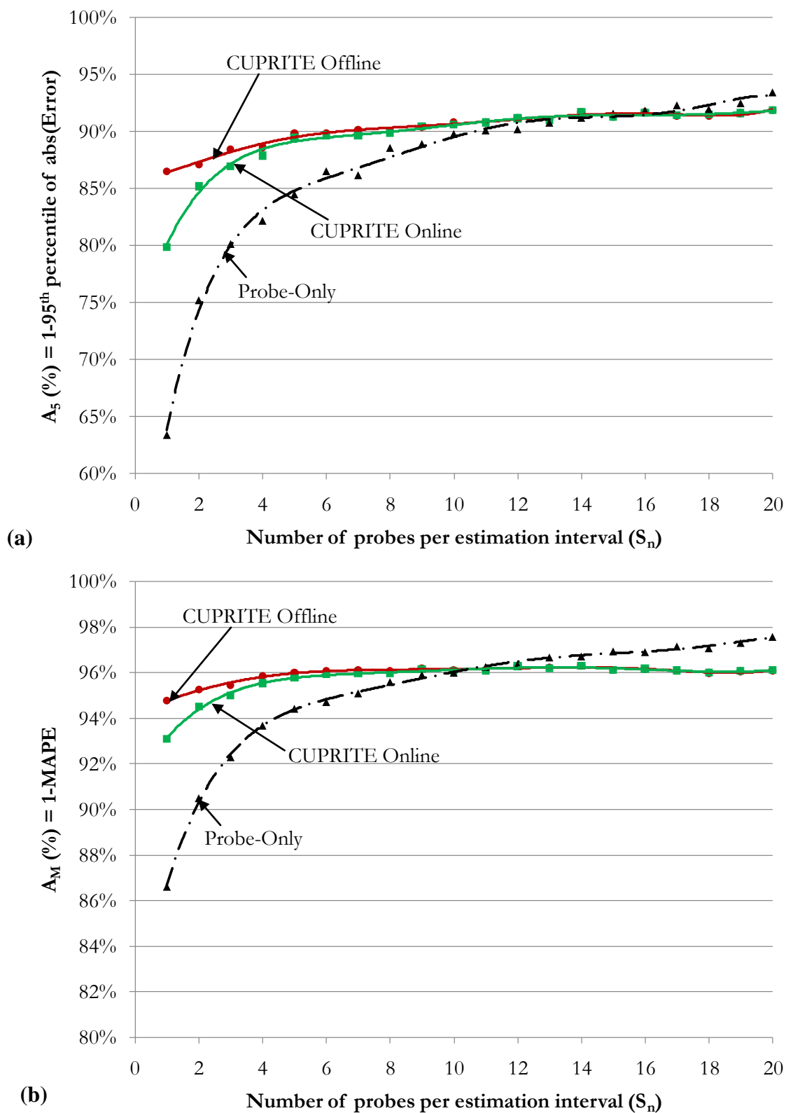
Figure 3-26: Simultaneous presence of both sink and source. Case B4.1 (20% sink and 10% source). Results for accuracy: a) A_5 and b) A_M versus S_n .
