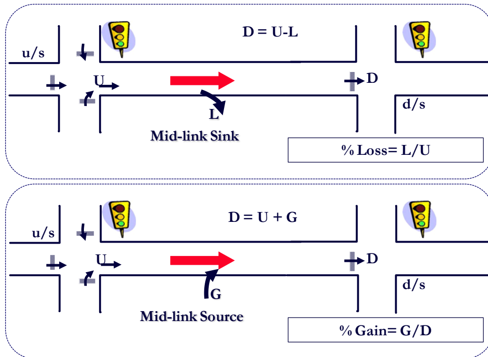
Figure 3-13: Definition of percentage loss to mid-link sink and percentage gain from mid-link source.
