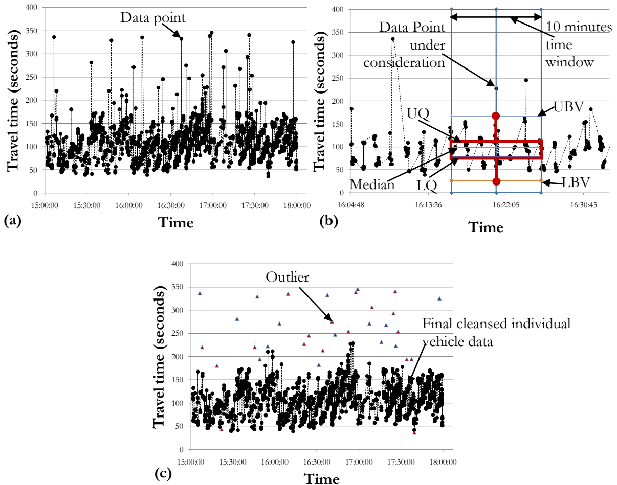
Figure 5-6: Example of filtering the outlier using box-and-whisker plot.
