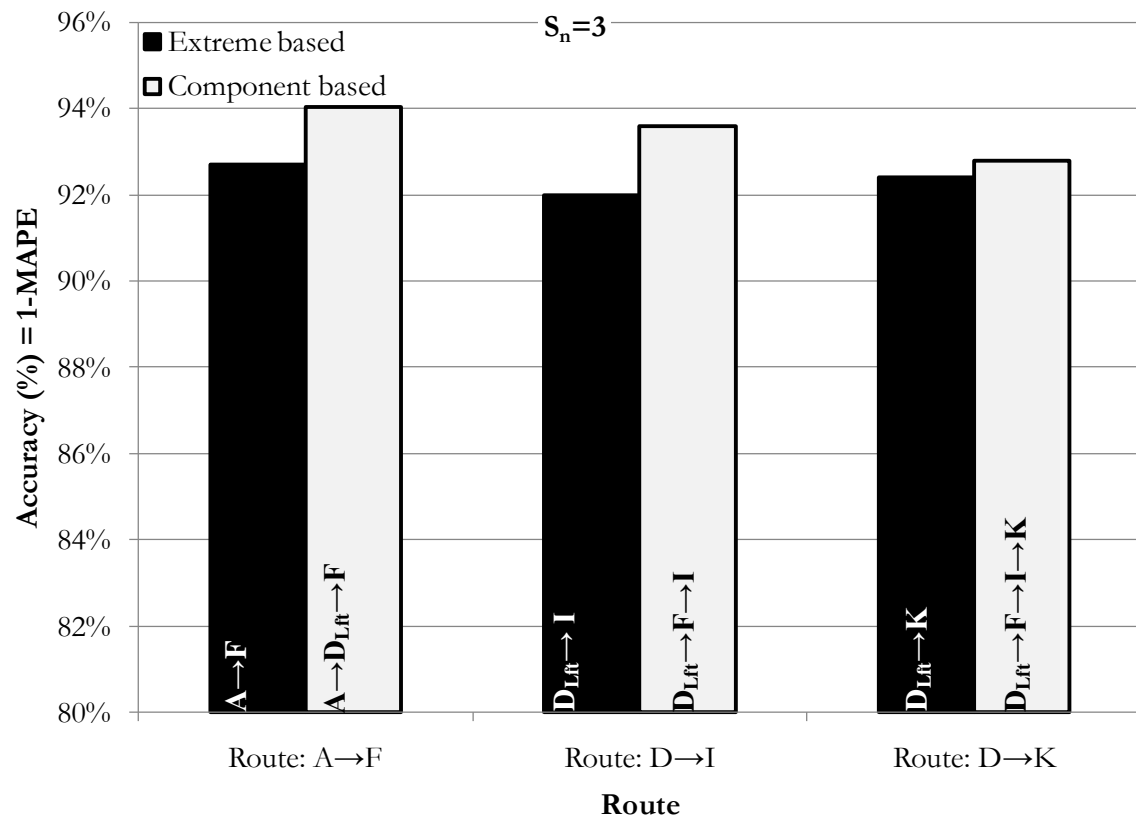
Figure 5-30: Results of Extreme based and Component based travel time estimation for different routes with S_n = 3 .
