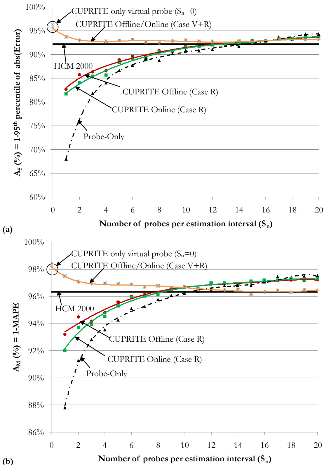
Figure C-2: Comparative results for 10% upstream detector overcounting during undersaturated traffic condition. Results for accuracy: (a) A_5 and (b) A_M versus S_n .
