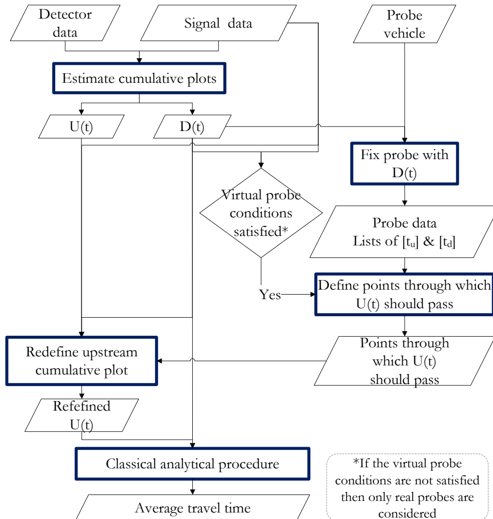
Figure 3-5: CUPRITE basic architecture.
