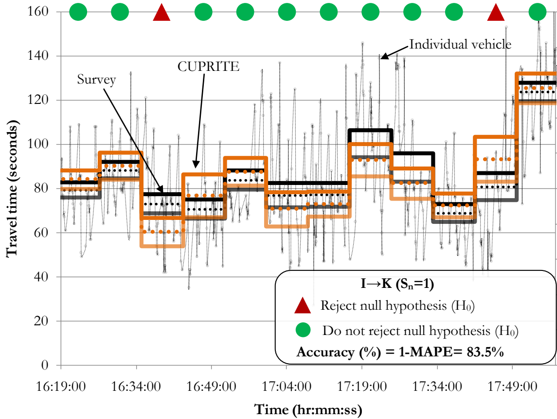
Figure 5-25: Results for I→K with S_n = 1 .
