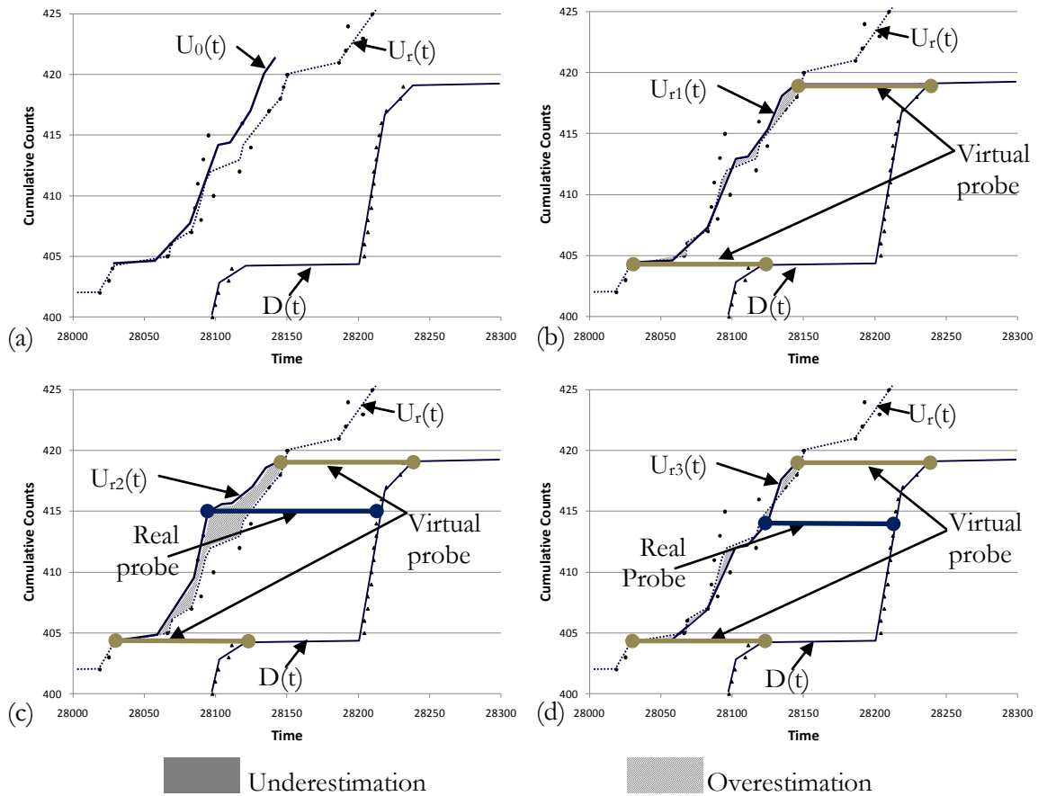
Figure 3-18: An example from 10 % mid-link sink case with different probe consideration.
