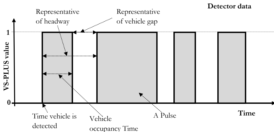
Figure 5-7: Pulse data representation for VS-PLUS detector data.
