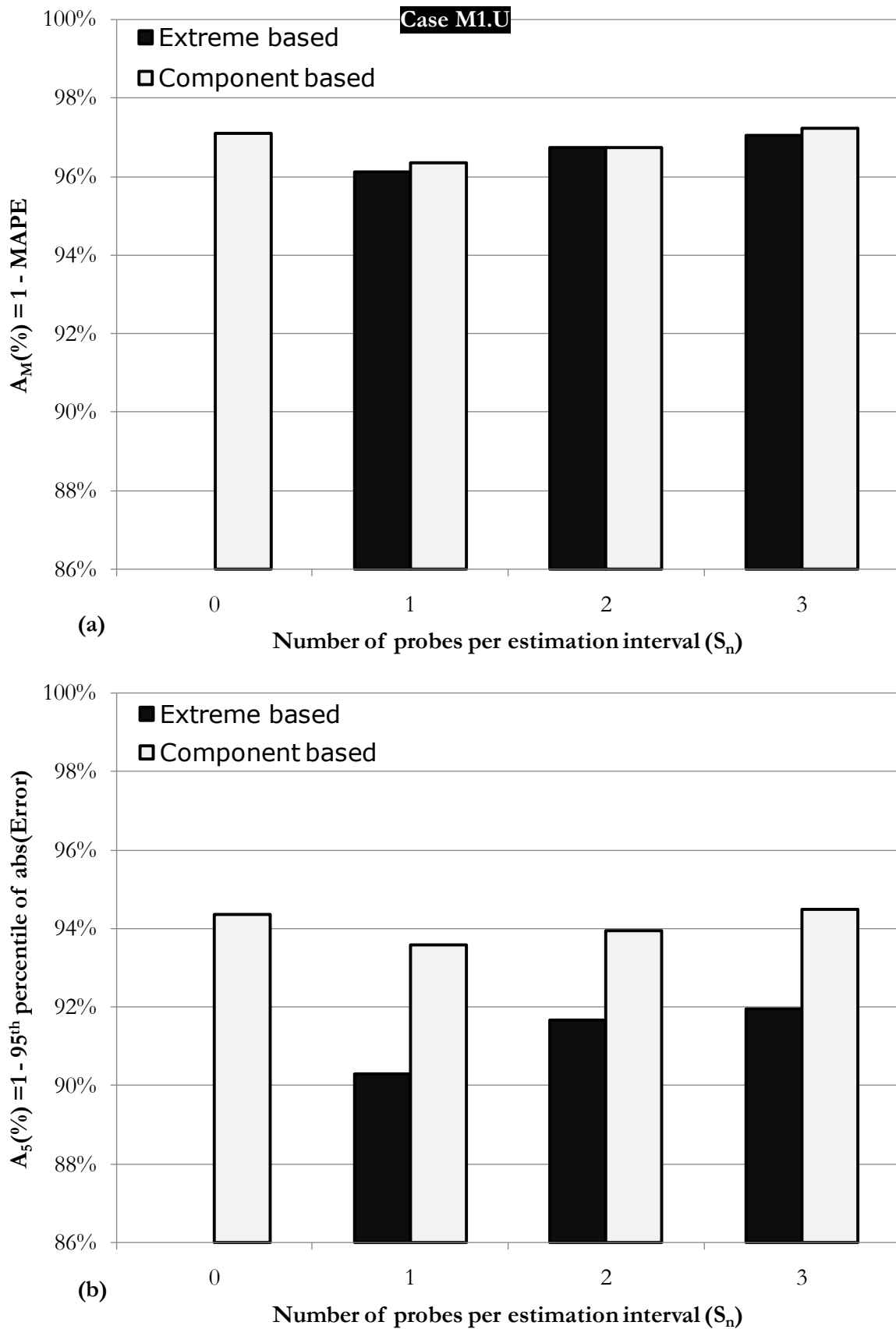
Figure 4-13: Case Study M1.U, Flow = F1, Accuracy (a) A_M and (b) A_5 versus S_n .
