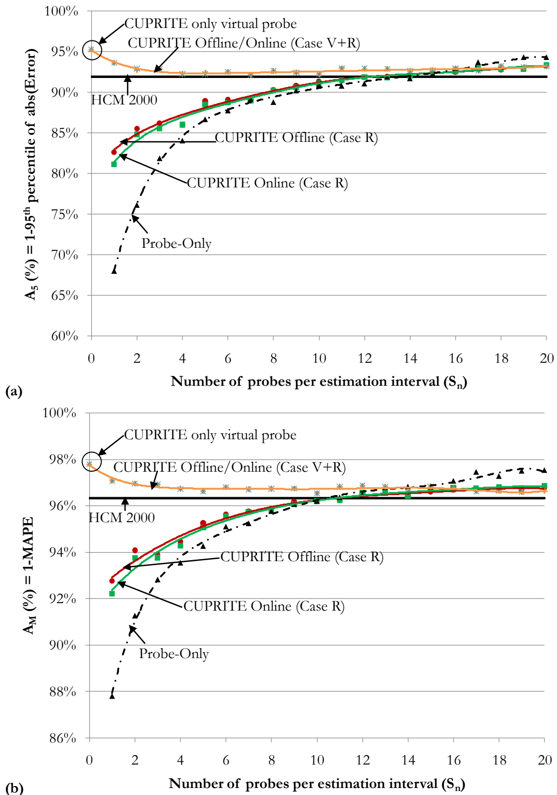
Figure C-3: Comparative results for 10% upstream detector undercounting case during undersaturated traffic condition. Results for accuracy: (a) A_5 and (b) A_M versus S_n .
