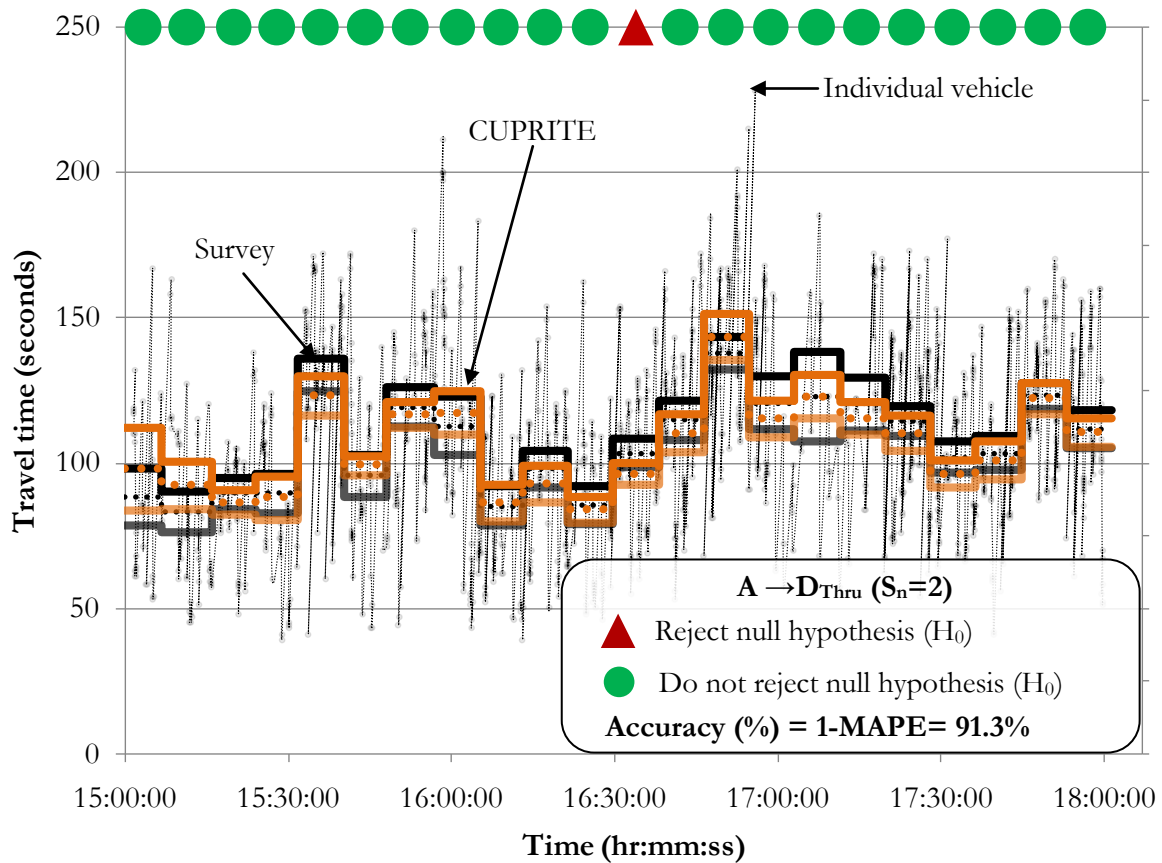
Figure 5-20: Results for A \rightarrow D Thru with S_n = 2 .
