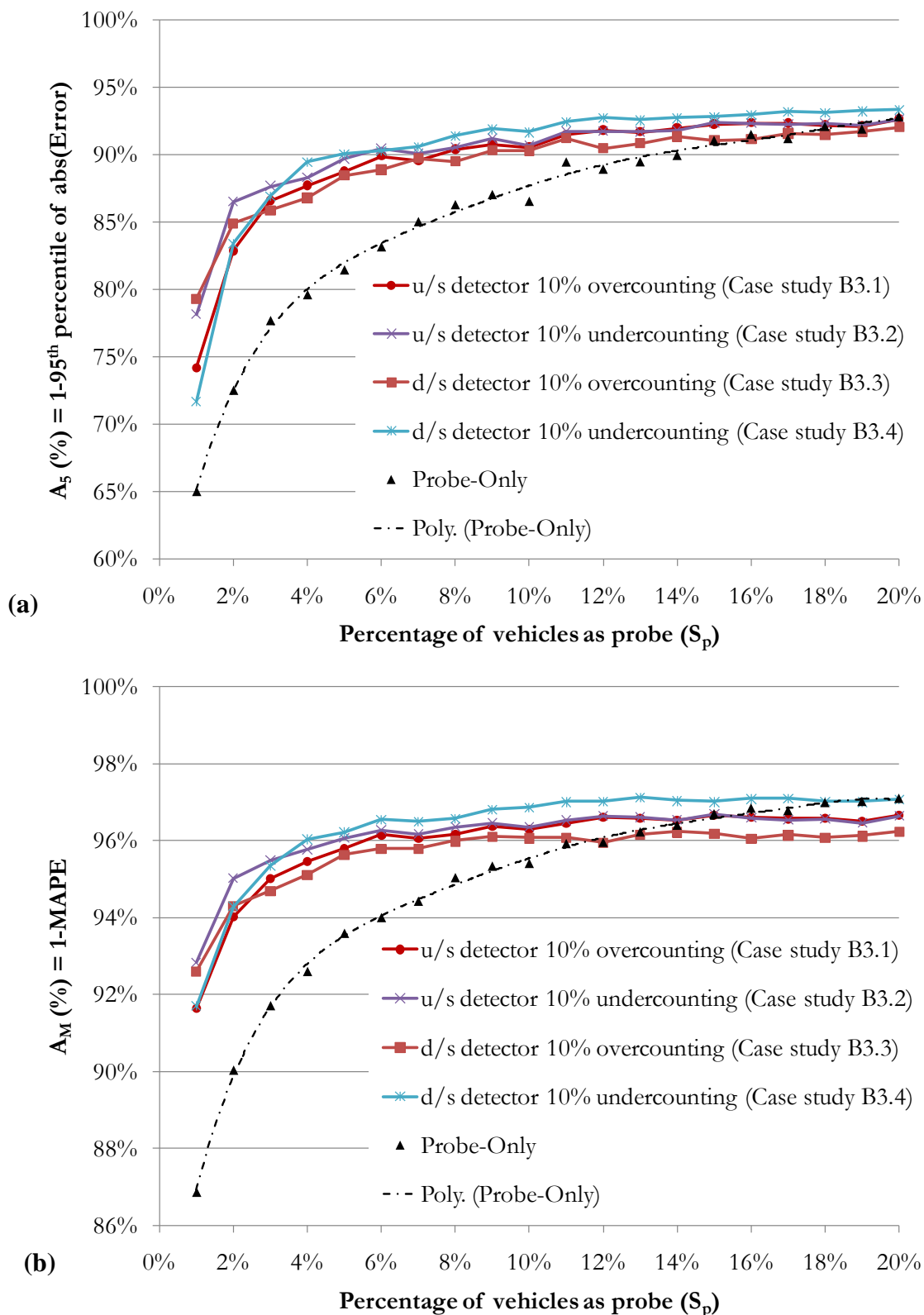
Figure C-12: Results for accuracy versus S_p case B3.1 to case B3.4 from CUPRITE online application.
