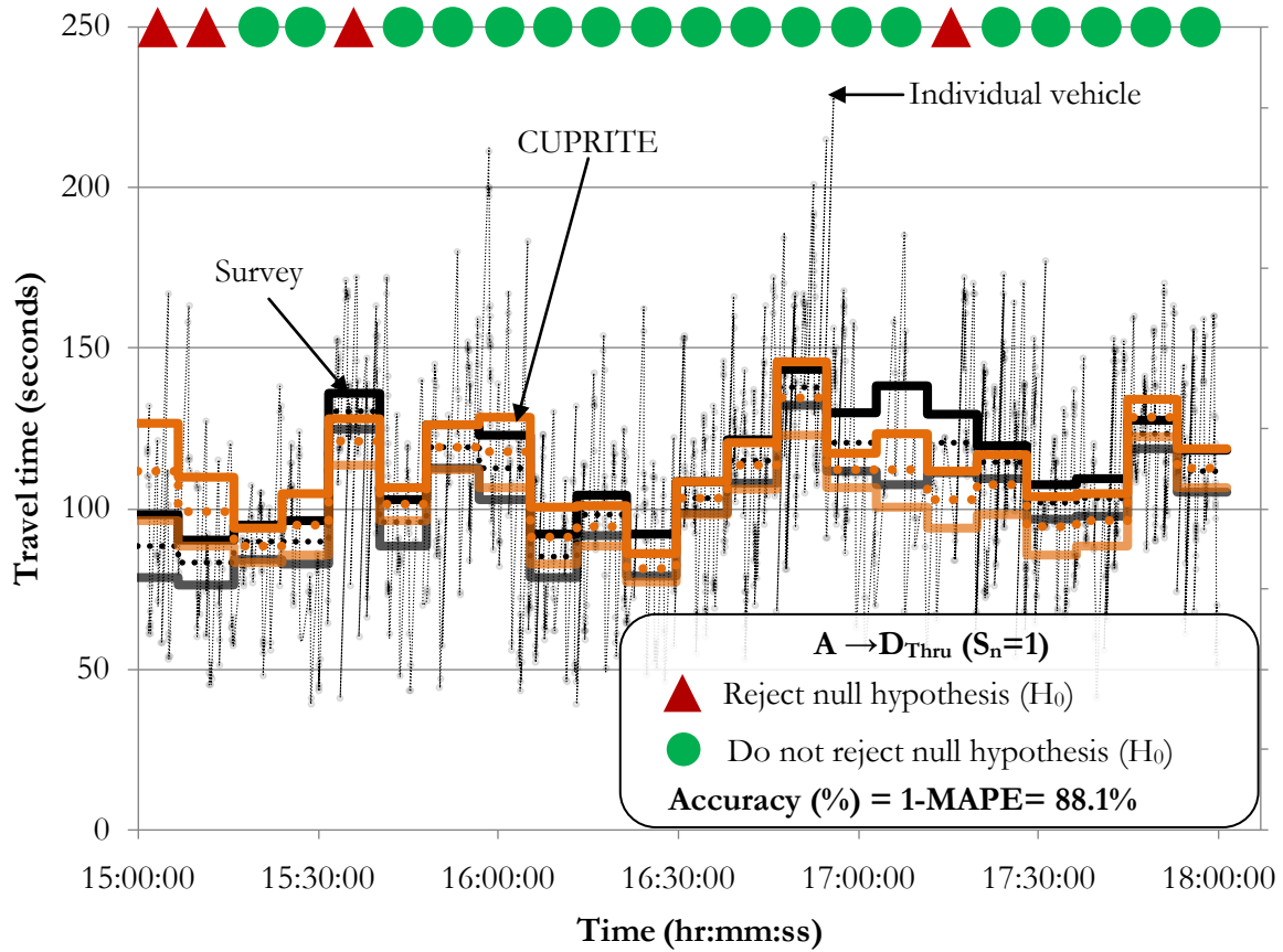
Figure 5-19: Results for A \rightarrow D Thru with S_n = 1 .
