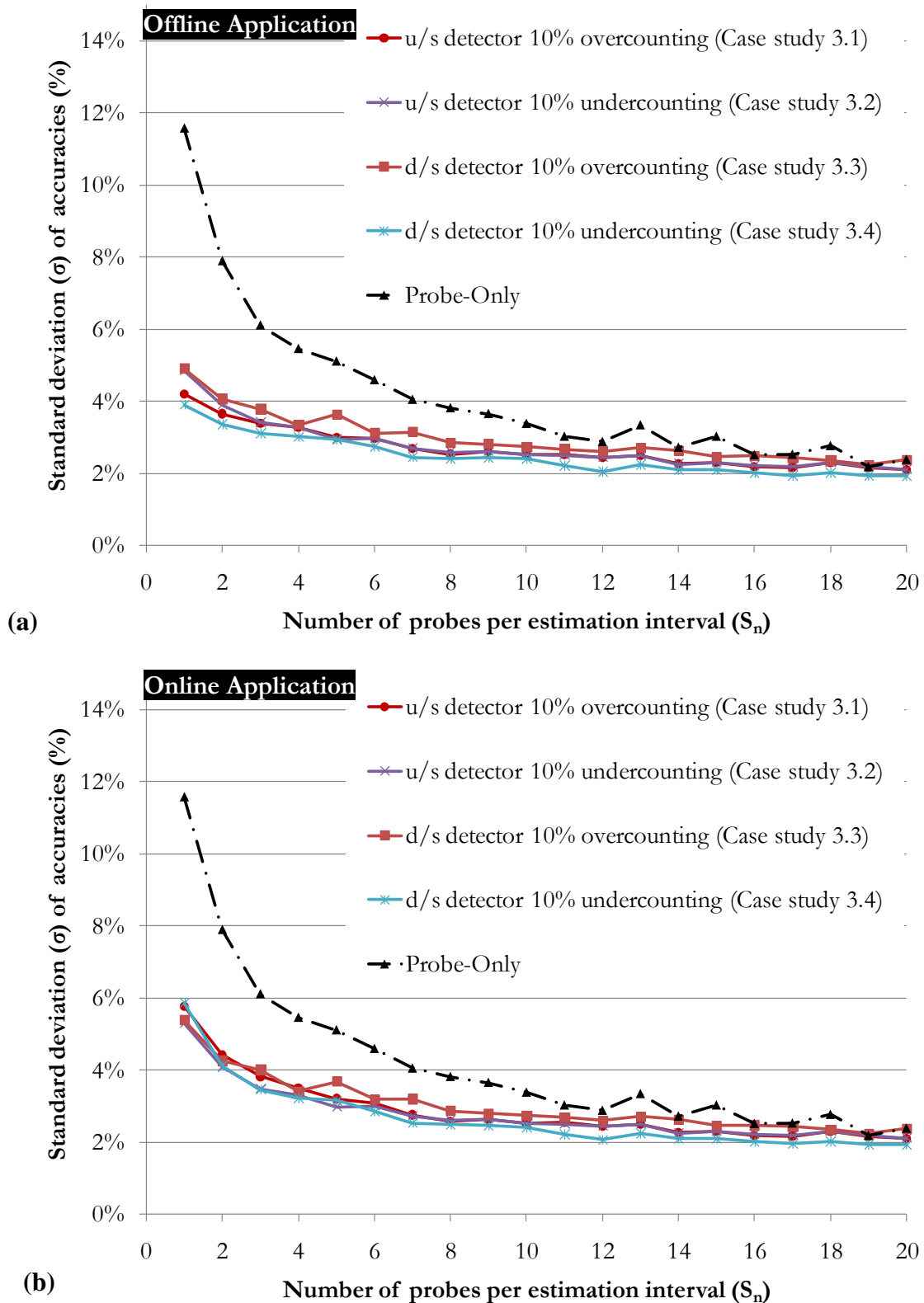
Figure C-9: Reliability of the estimate for case study (B3.1 to B3.4) on detector counting error with fixed number of probes per estimation interval ( S_n ) for a) Offline application and b) Online application.
