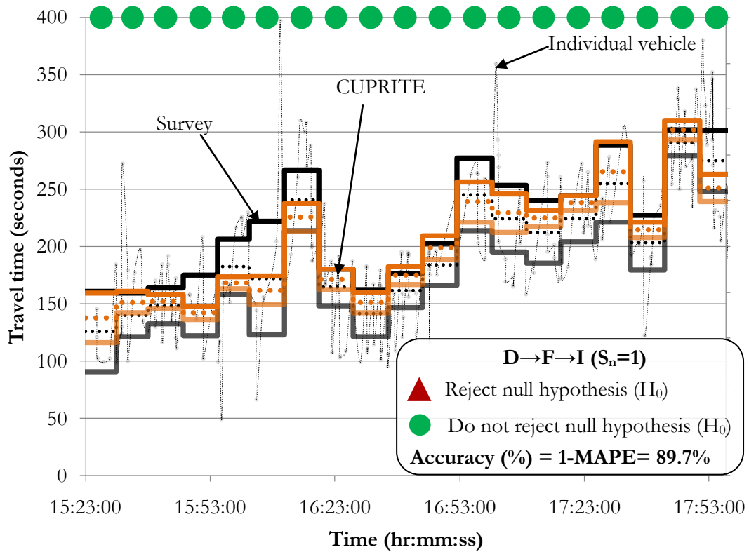
Figure E-5: Component based results for D→F→I ( S_n=1 ).
