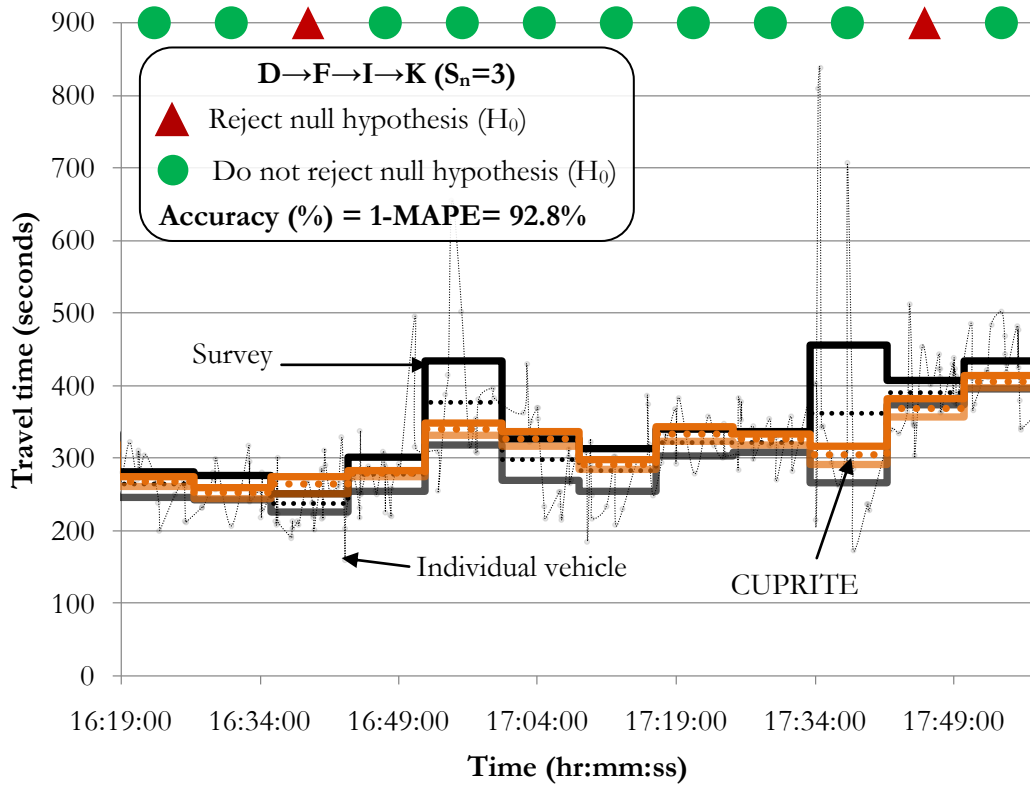
Figure F-6: Component based results for D→F→I→K ( S_n=3 ).
