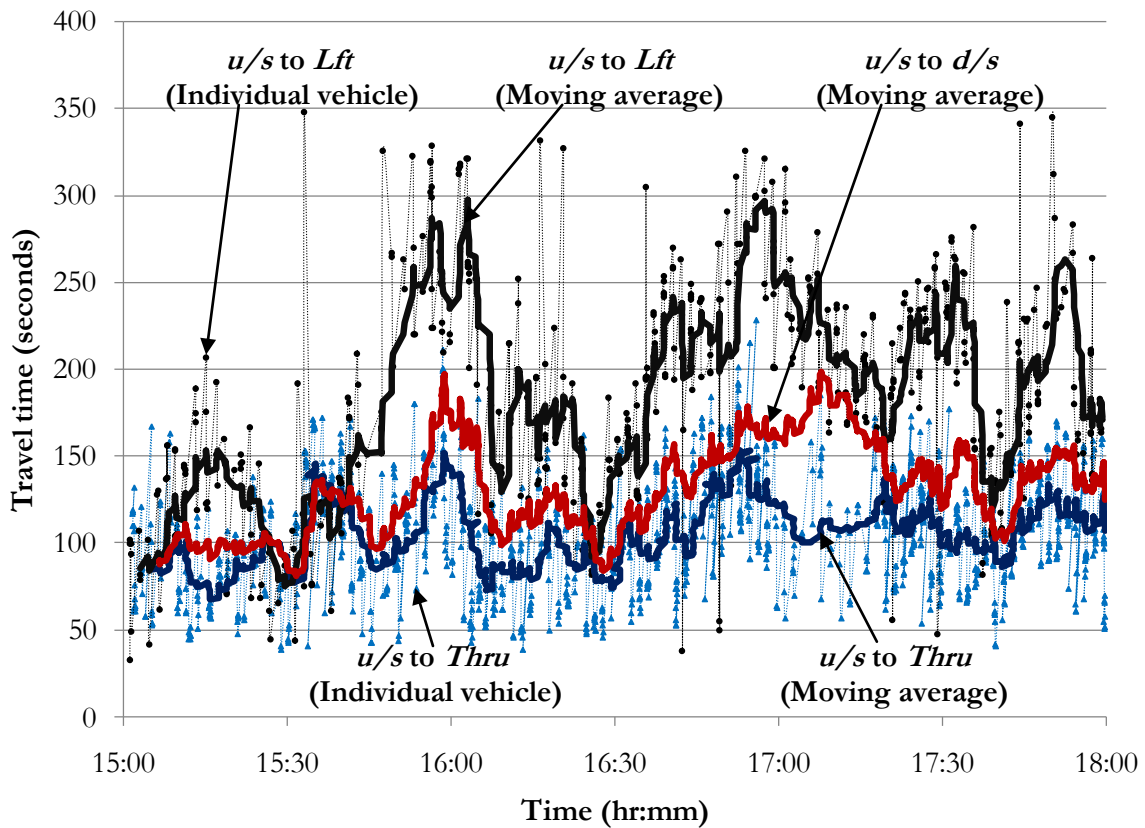
Figure 4-2: Example for actual travel time for different exit movements associated with a link.
