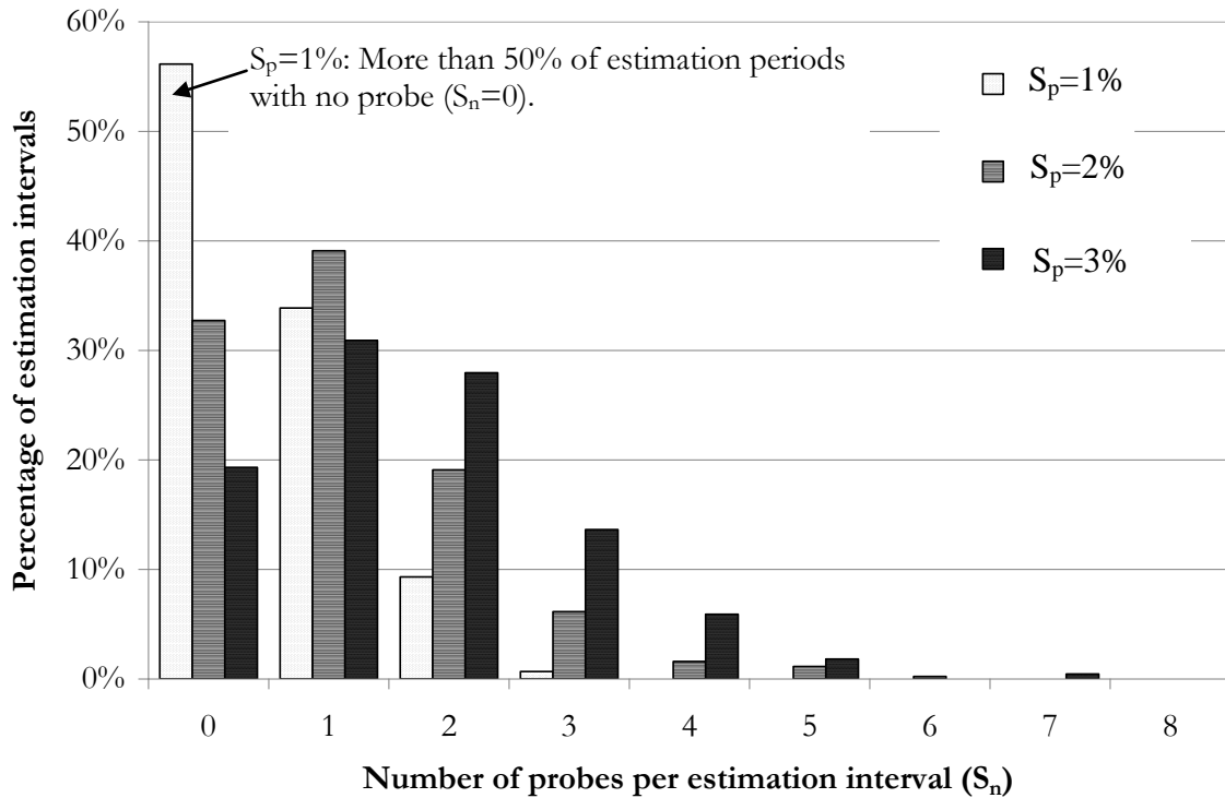
Figure 5-34: Percentage of estimation intervals versus S_n for route A \rightarrow D_{Lft} .
