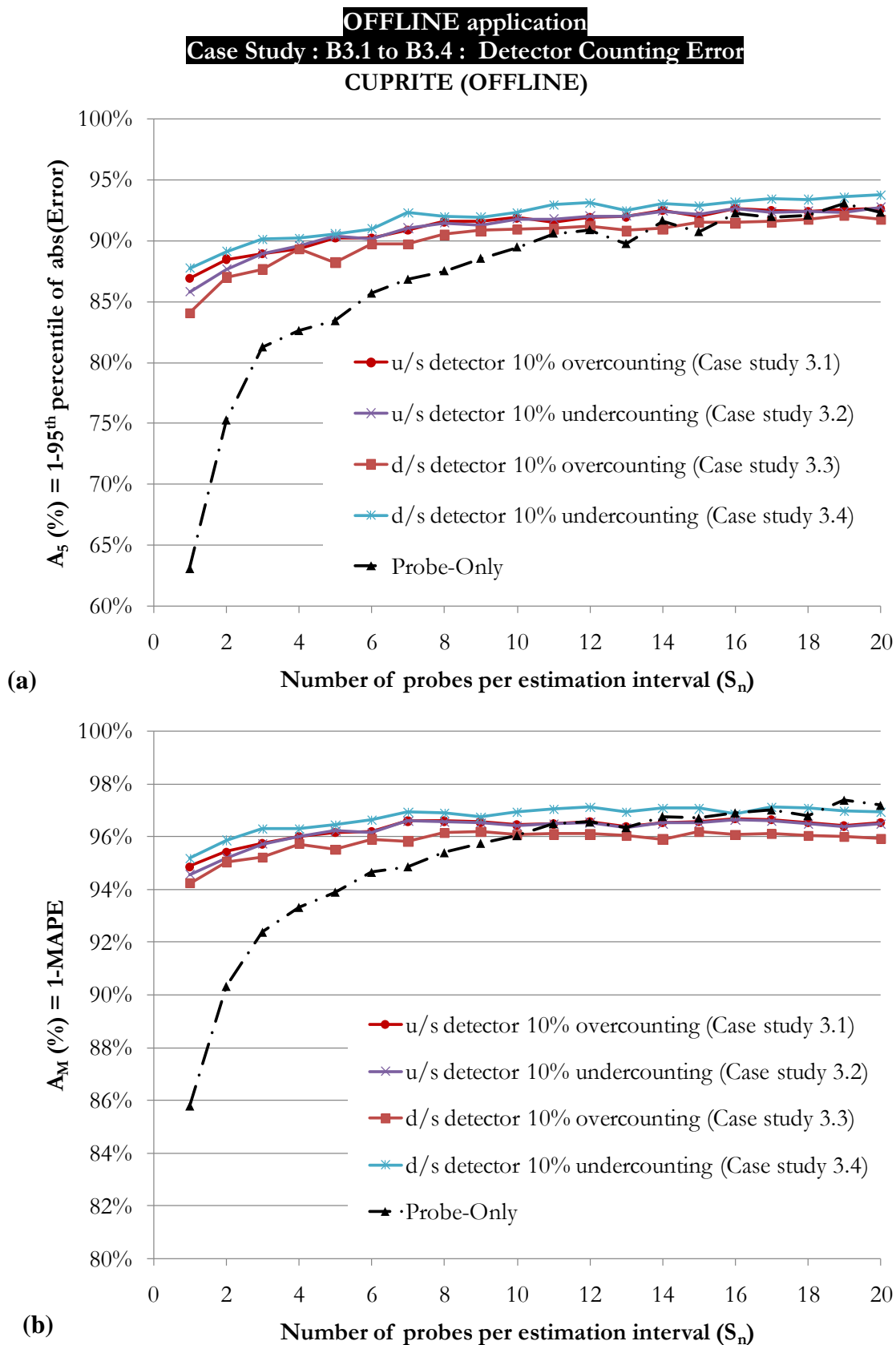
Figure 3-25: Detector counting error with fixed number of probes per estimation interval ( S_n ) for offline application: Cases B3. 1 to B3.4: Results for accuracy: a) A_5 and b) A_M versus S_n .
