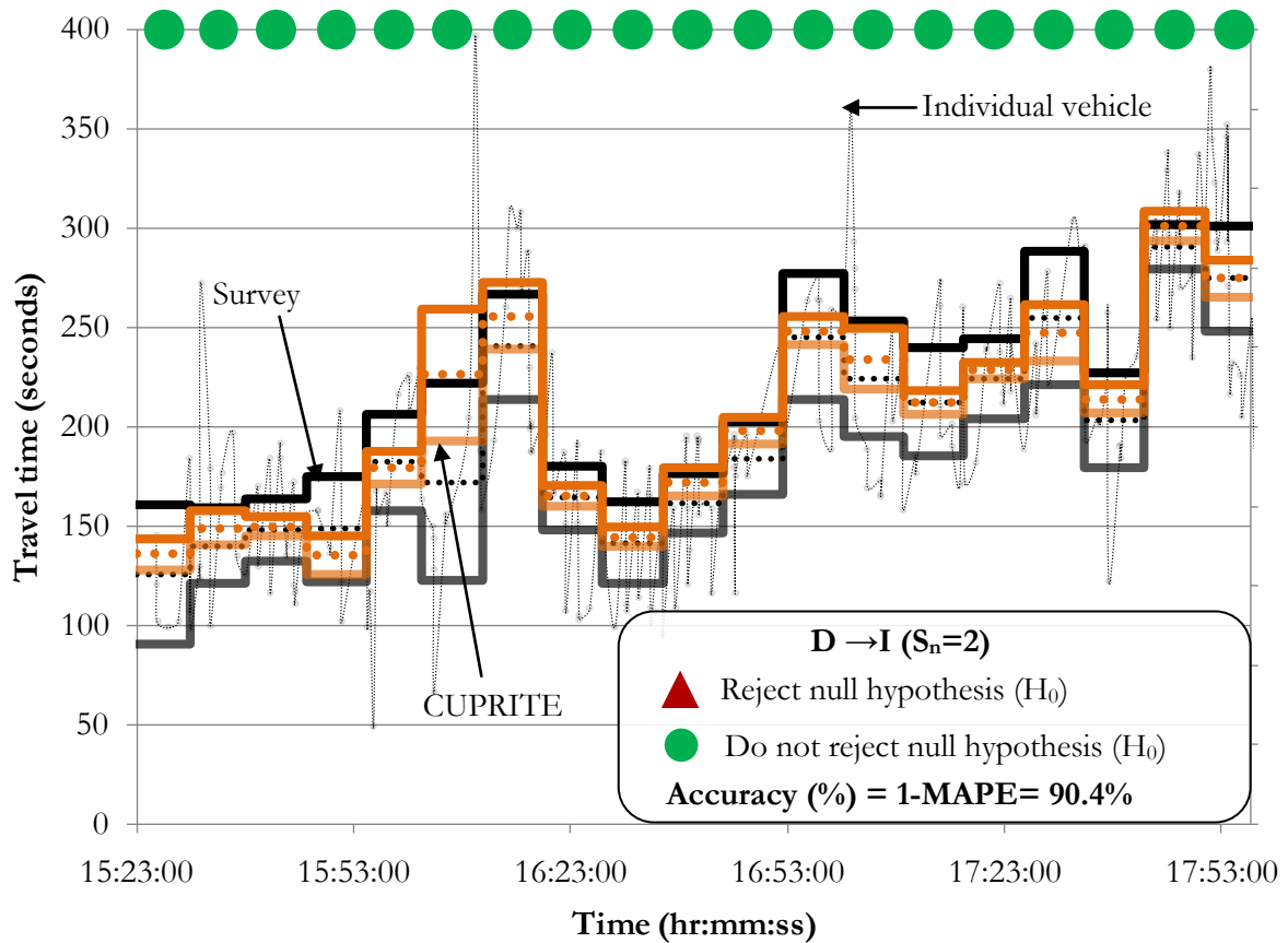
Figure 5-23: Results for D→I with S_n = 2 .
