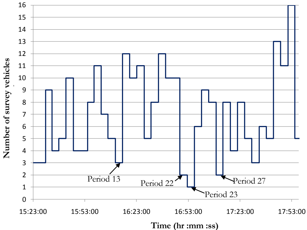
Figure E-1: Number of survey vehicles in estimation interval of 5 times the signal cycle.
