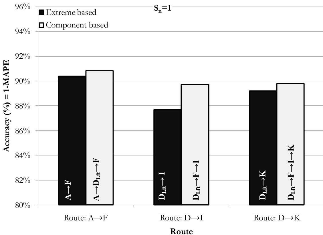
Figure 5-28: Results of Extreme based and Component based travel time estimation for different routes with S_n = 1 .
