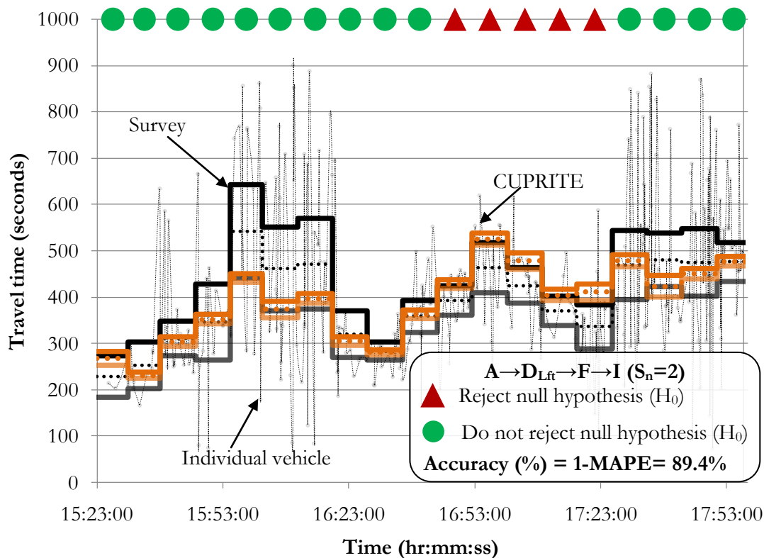
Figure G-5: Component based results for A→D Lft →F→I ( S_n=2 ).
