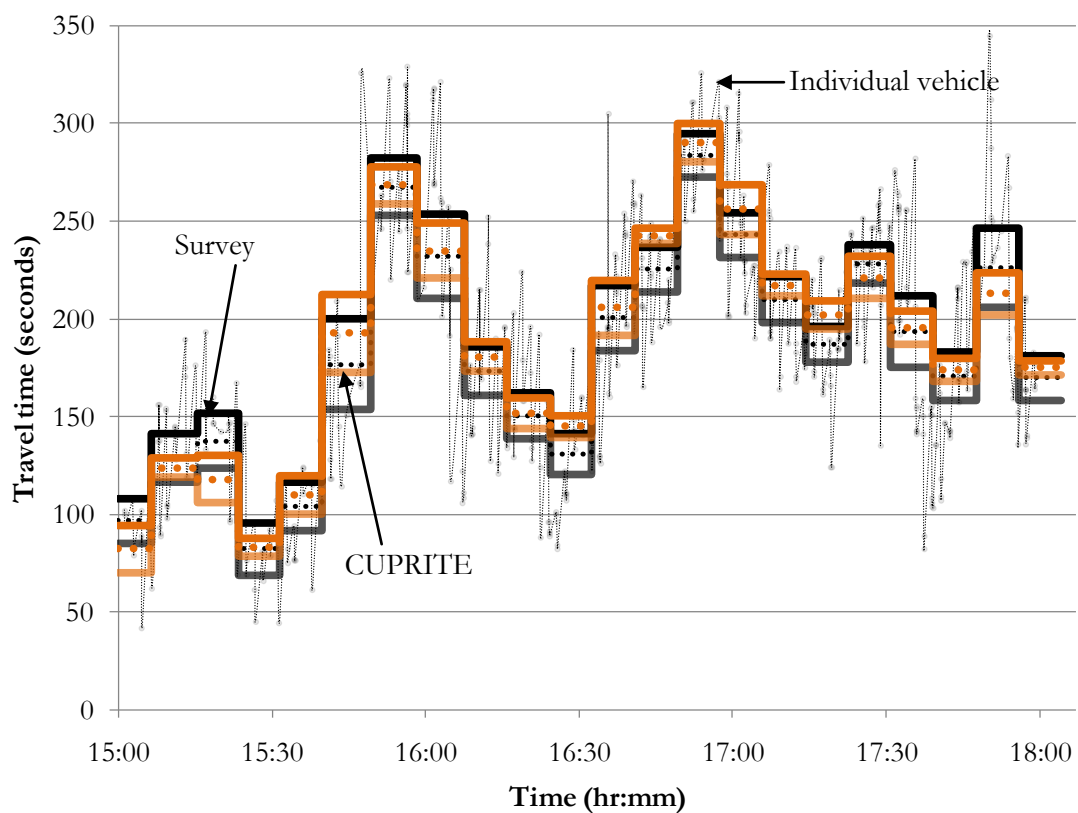
Figure 0-4: Results for A \rightarrow D_{Lft} with S_n = 1 .
