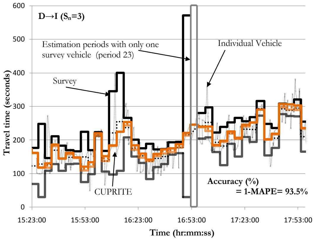
Figure E-4: Extreme based results for D→I ( S_n=3 ).
