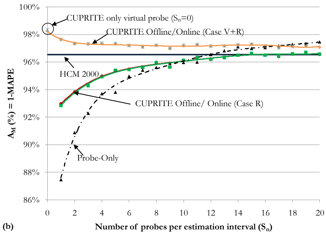
Figure 3-16: Comparative results for 10% mid-link sink case during undersaturated traffic condition. (a) Results for accuracy: A_5 and (b) Results for accuracy: A_M .
