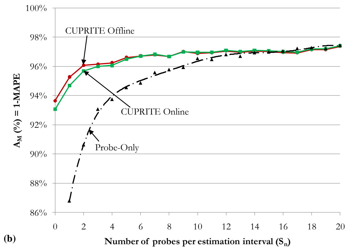
Figure 3-27: Simultaneous presence of both sink and source. Case B4.3 (10% sink and 10% source). Results for accuracy: a) A_5 and b) A_M versus S_n .
