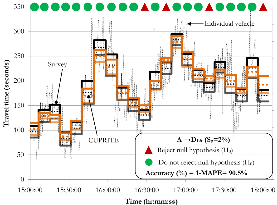
Figure 5-32: Results for A→D Lft with S_p=2\% .
