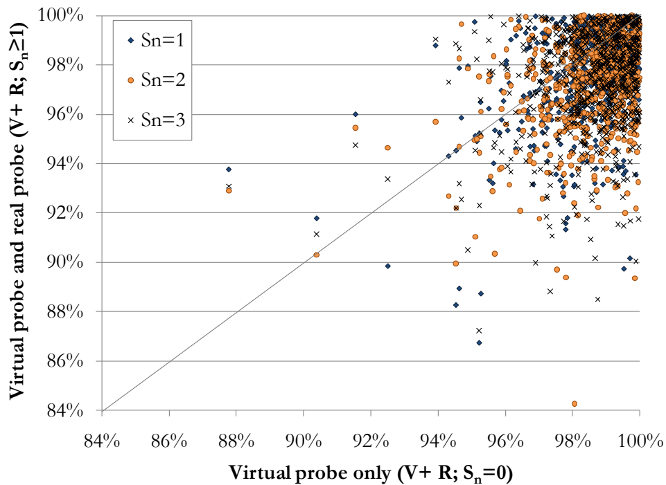
Figure 3-19: Accuracy estimates ( A_5 ) from V+R case with S_n=1, 2 and 3 probes versus S_n=0 from 10% mid-link sink (case A3.1).
