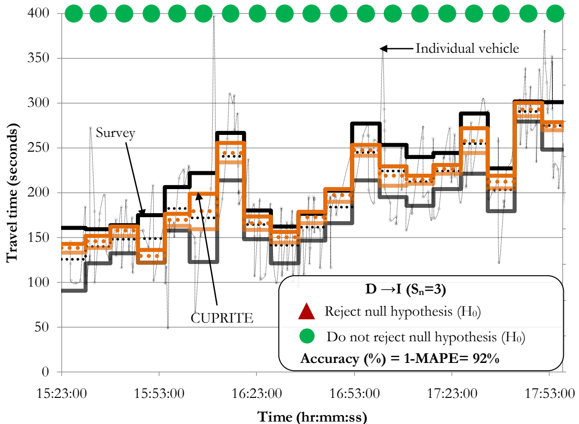
Figure 5-24: Results for D→I with S_n = 3 .
