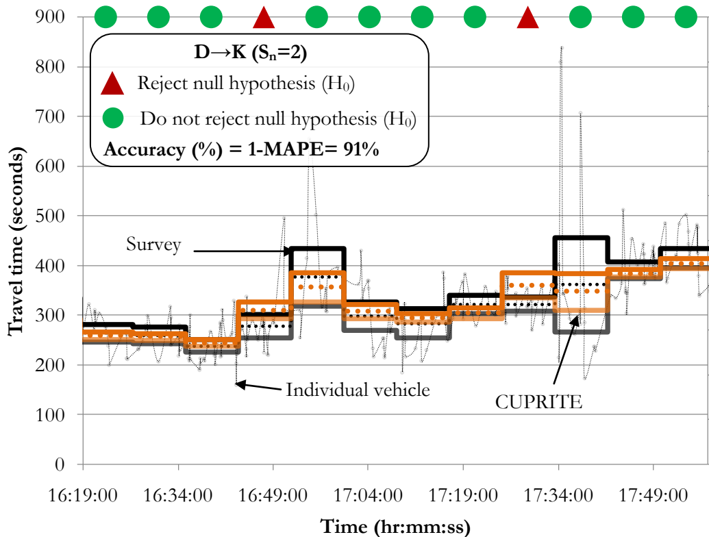
Figure F-2: Extreme based results for D→K ( S_n=2 ).
