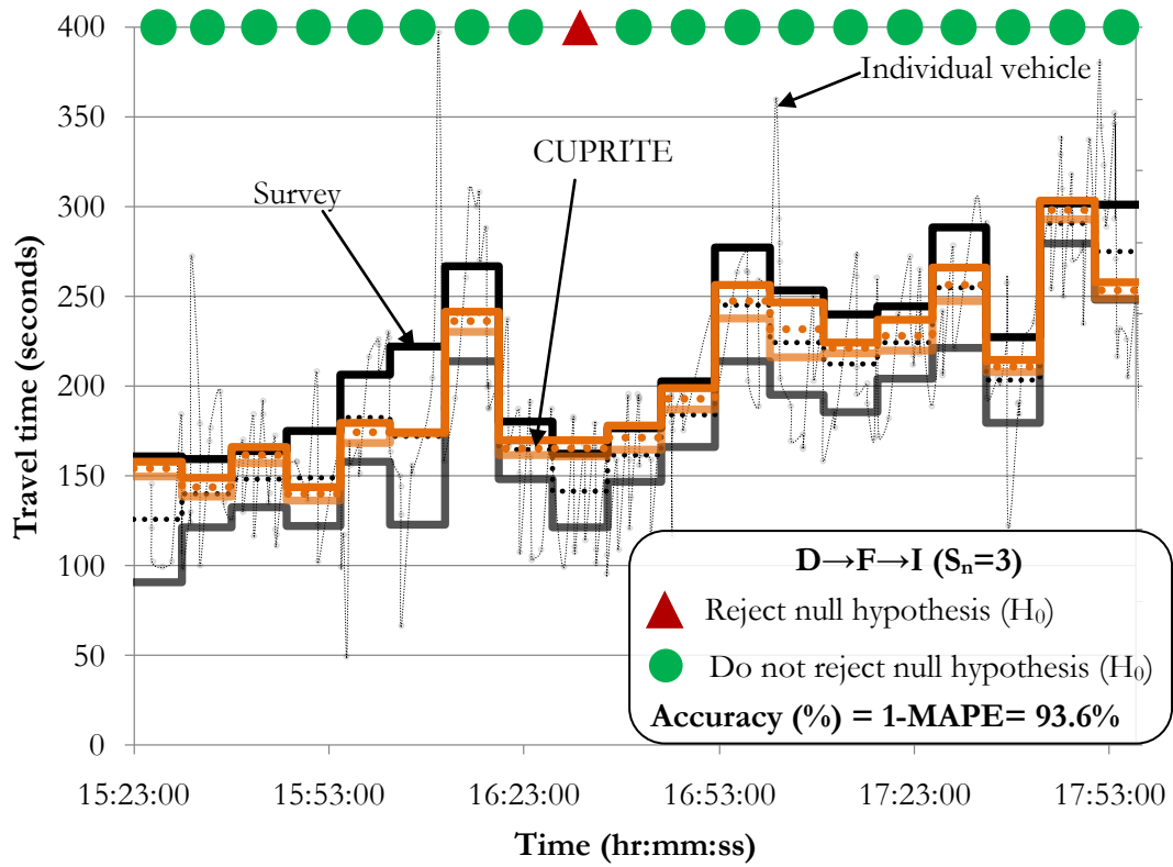
Figure E-7: Component based results for D→F→I (S n =3).
