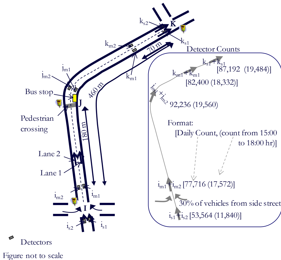
Figure 5-15: Illustration of the link characteristics between intersections I and K and corresponding detector count.
