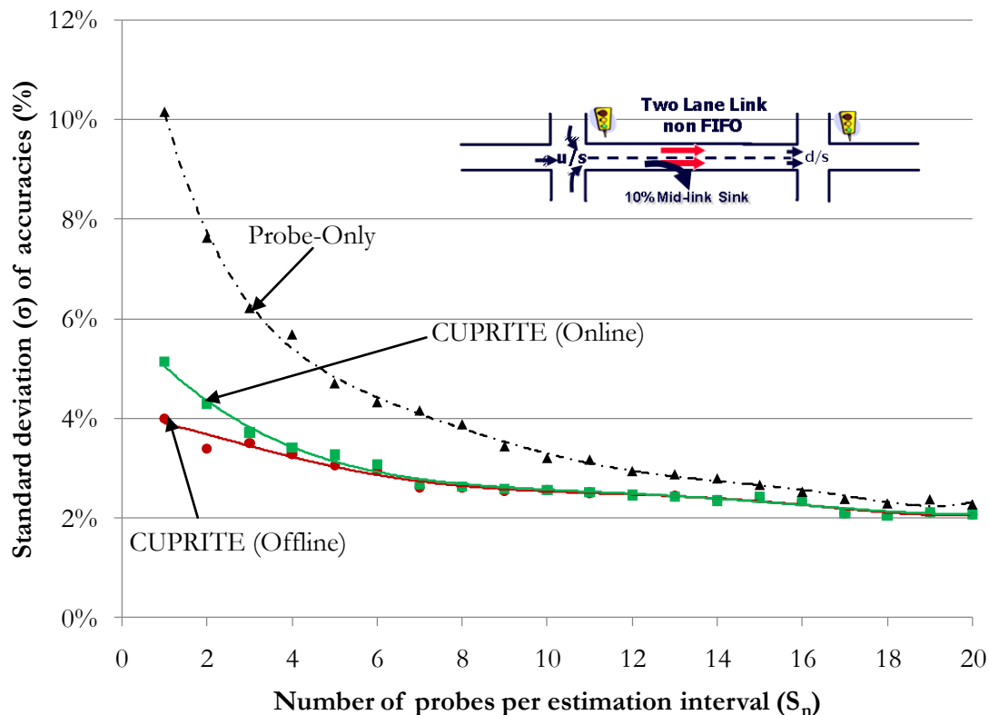
Figure 3-28: Standard deviation of accuracy versus number of probes per estimation interval.
